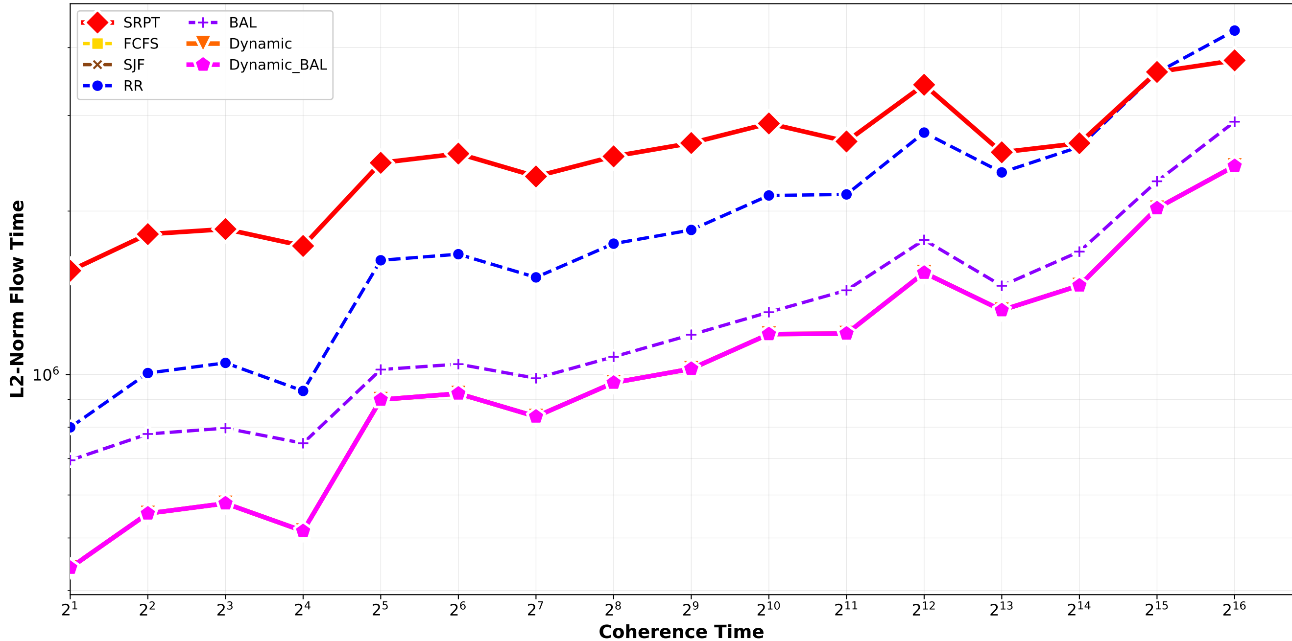
Clairvoyant Algorithms - L2 Norm Flow Time normal_combination_softrandom std6_std9_std12_std15 / quadruplet_1
