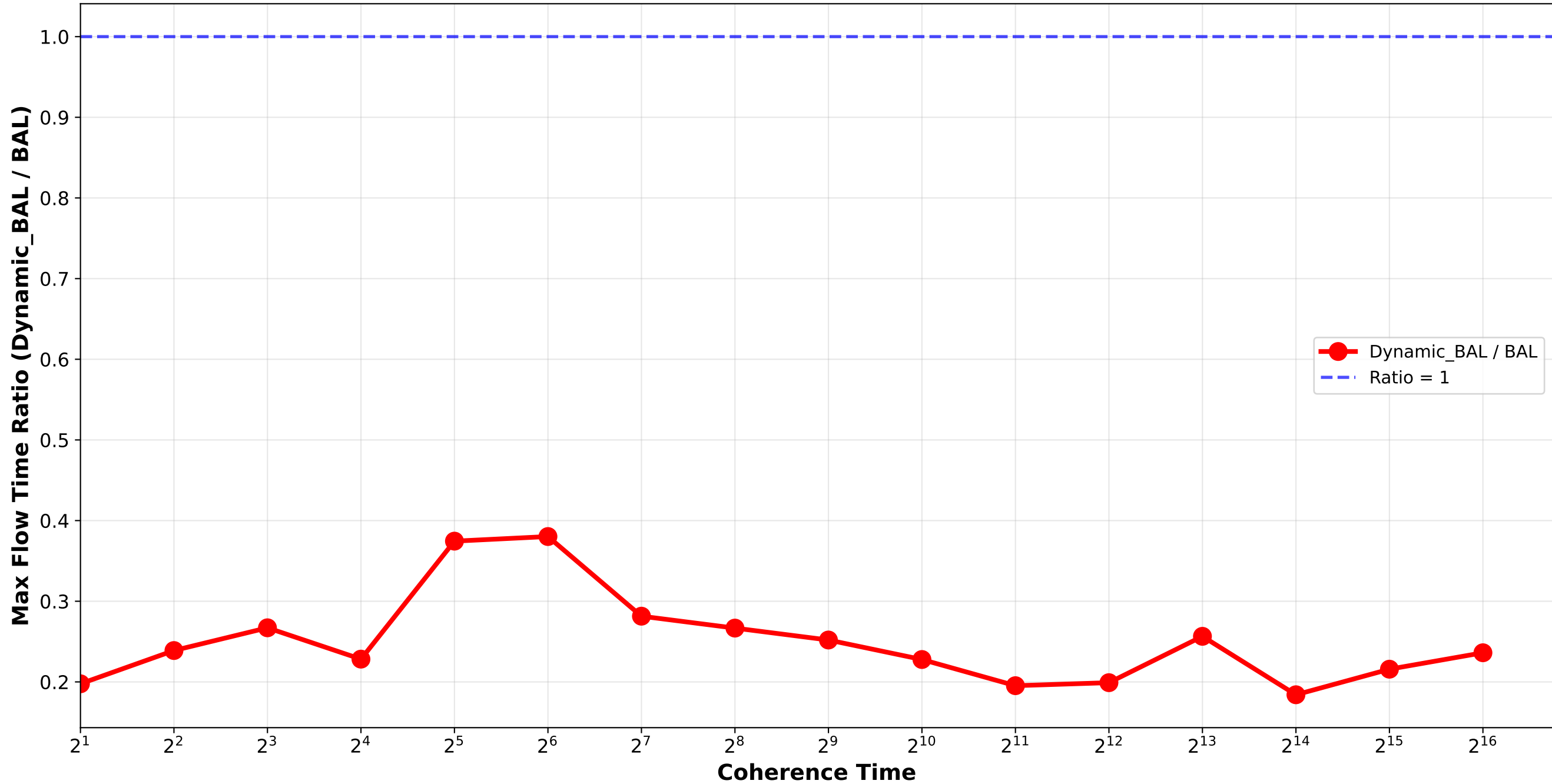
Dynamic_BAL vs BAL - Max Flow Time Ratio normal_combination_softrandom std6_std9_std12_std15 / quadruplet_1
