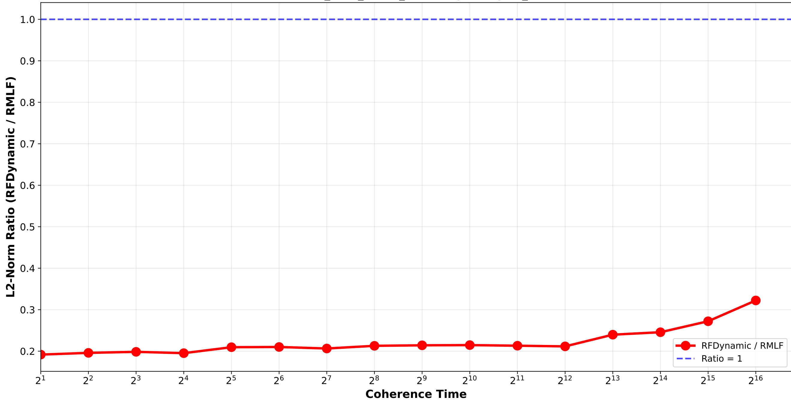
RFDynamic vs RMLF - L2 Norm Ratio normal_combination_softrandom std6_std9_std12_std15 / quadruplet_1
