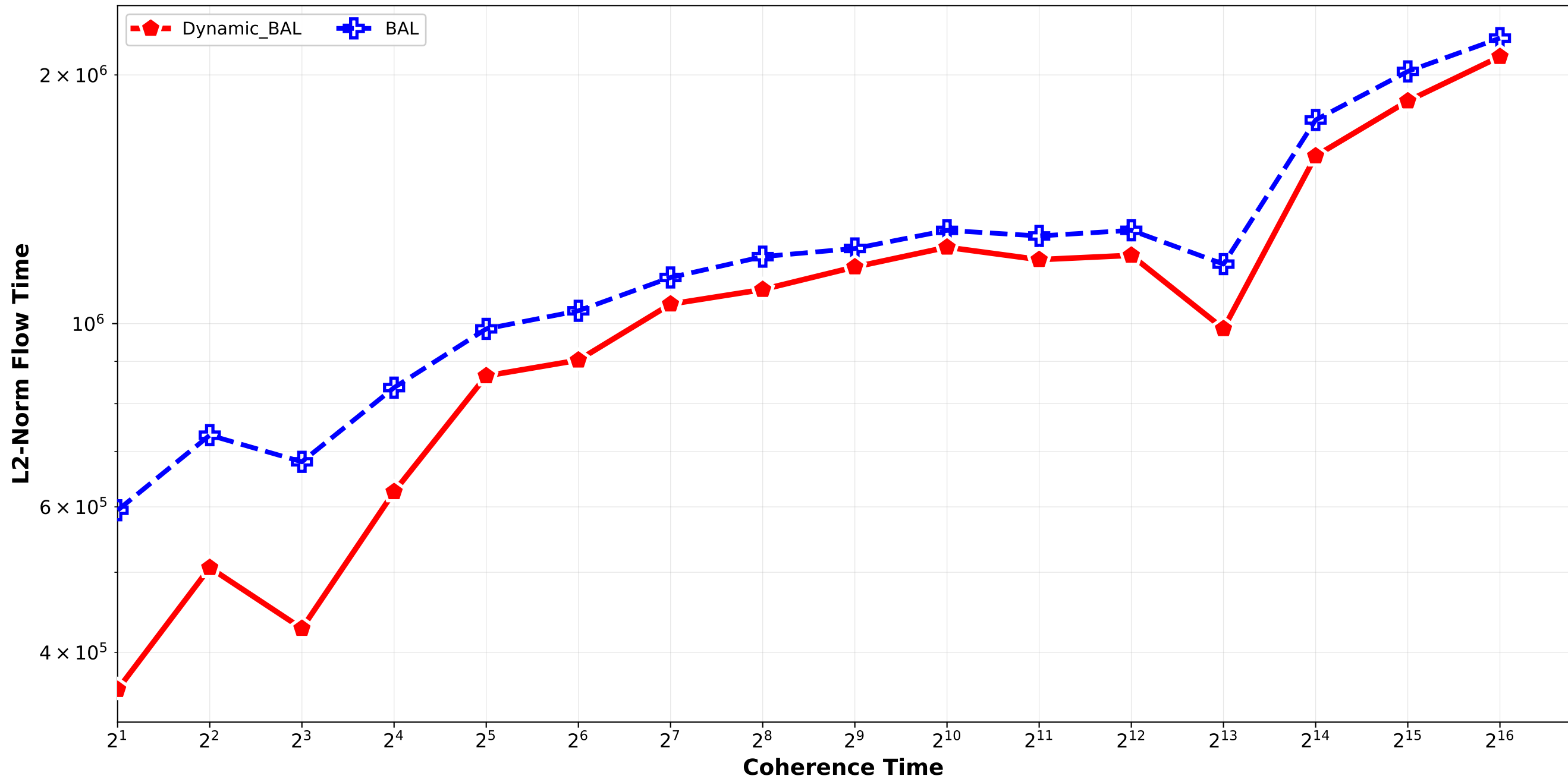
Dynamic_BAL vs BAL - L2 Norm Flow Time normal_combination_softrandom std9_std12_std15_std18 / quadruplet_2
