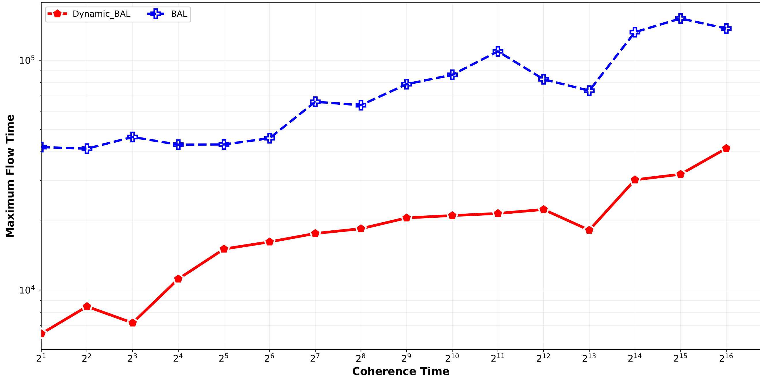
Dynamic_BAL vs BAL - Maximum Flow Time normal_combination_softrandom std9_std12_std15_std18 / quadruplet_2
