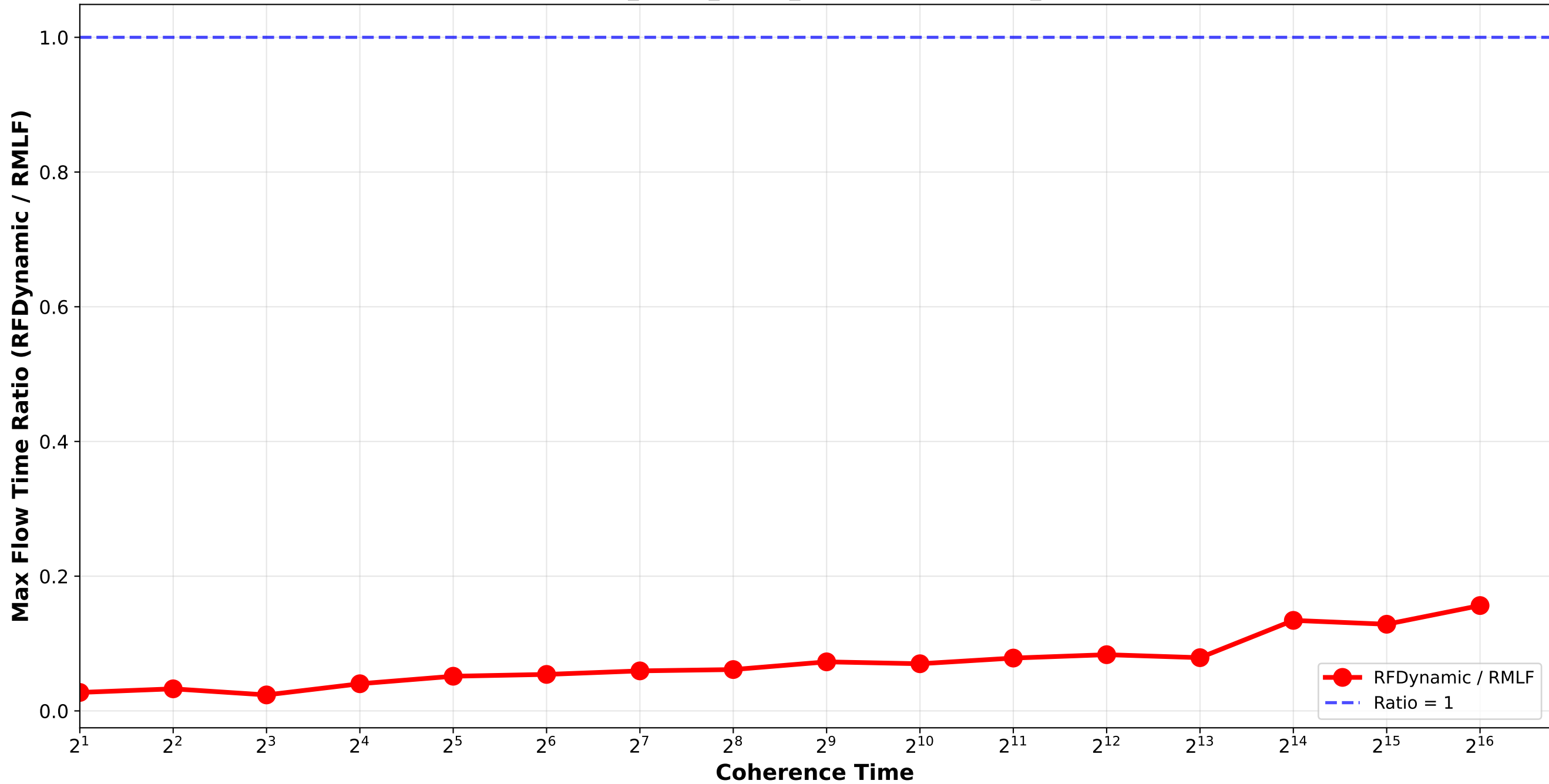
RFDynamic vs RMLF - Max Flow Time Ratio normal_combination_softrandom std9_std12_std15_std18 / quadruplet_2
