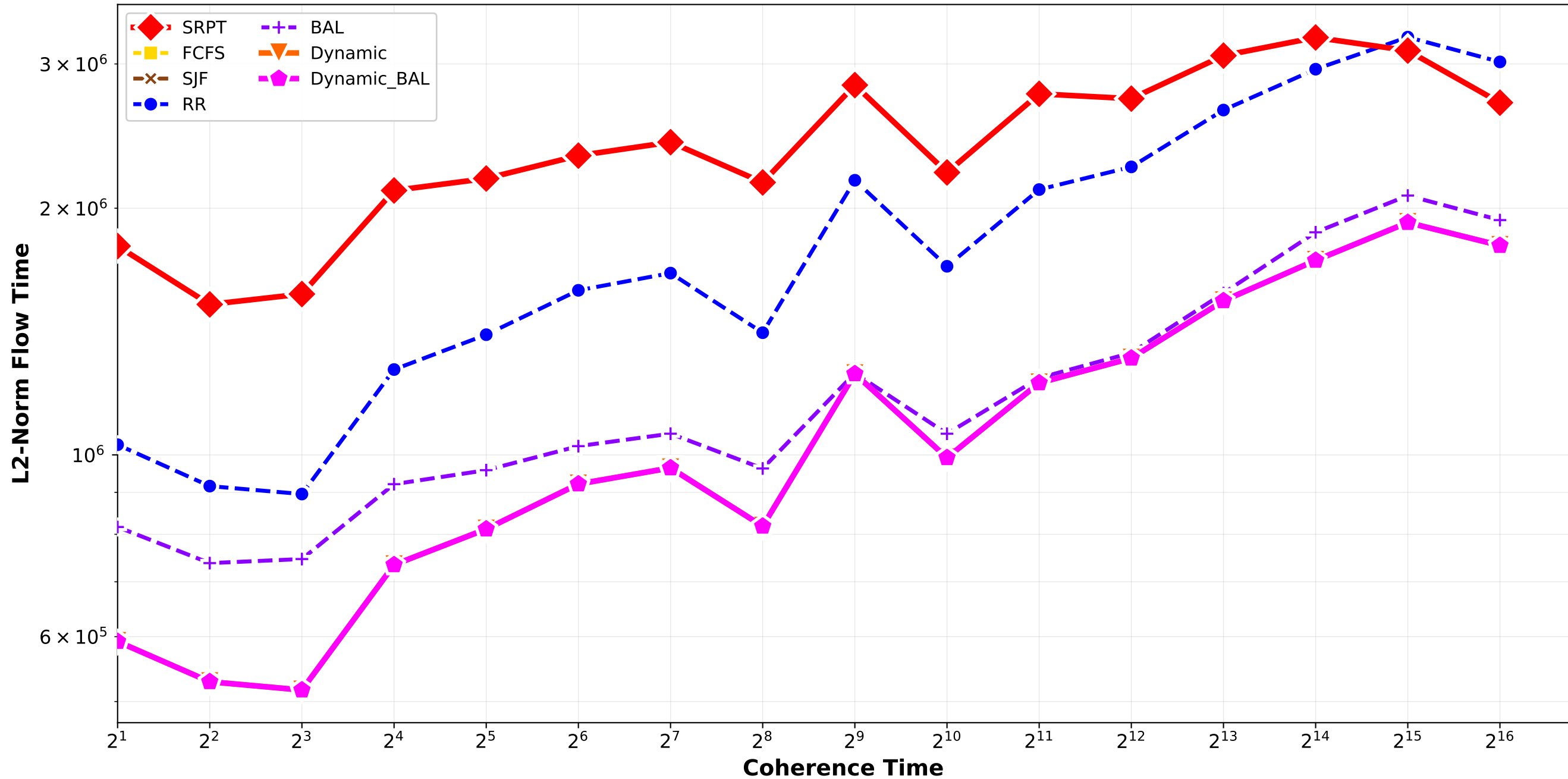
Clairvoyant Algorithms - L2 Norm Flow Time normal_combination_softrandom std12_std15_std18 / triplet_3
