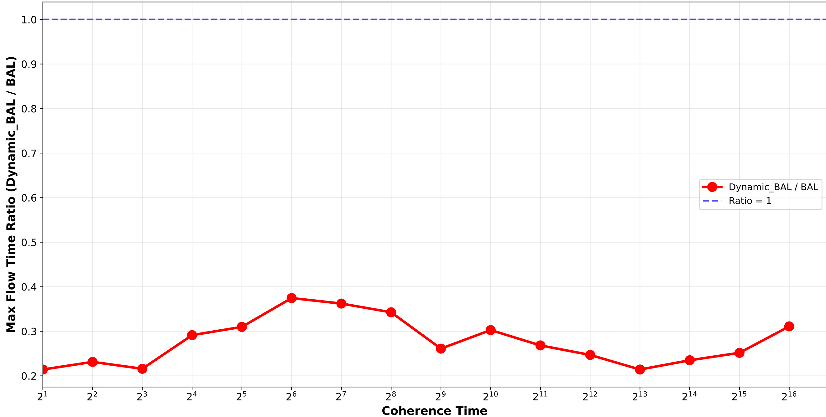
Dynamic_BAL vs BAL - Max Flow Time Ratio normal_combination_softrandom std12_std15_std18 / triplet_3
