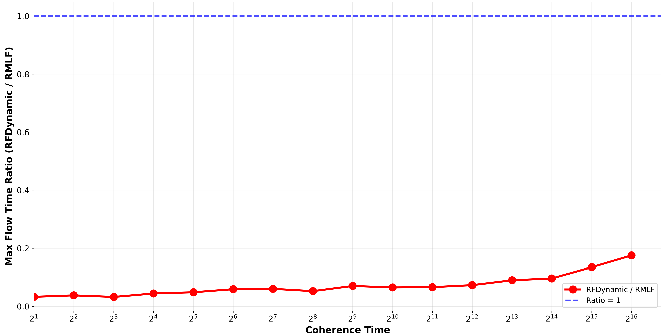
RFDynamic vs RMLF - Max Flow Time Ratio normal_combination_softrandom std12_std15_std18 / triplet_3
