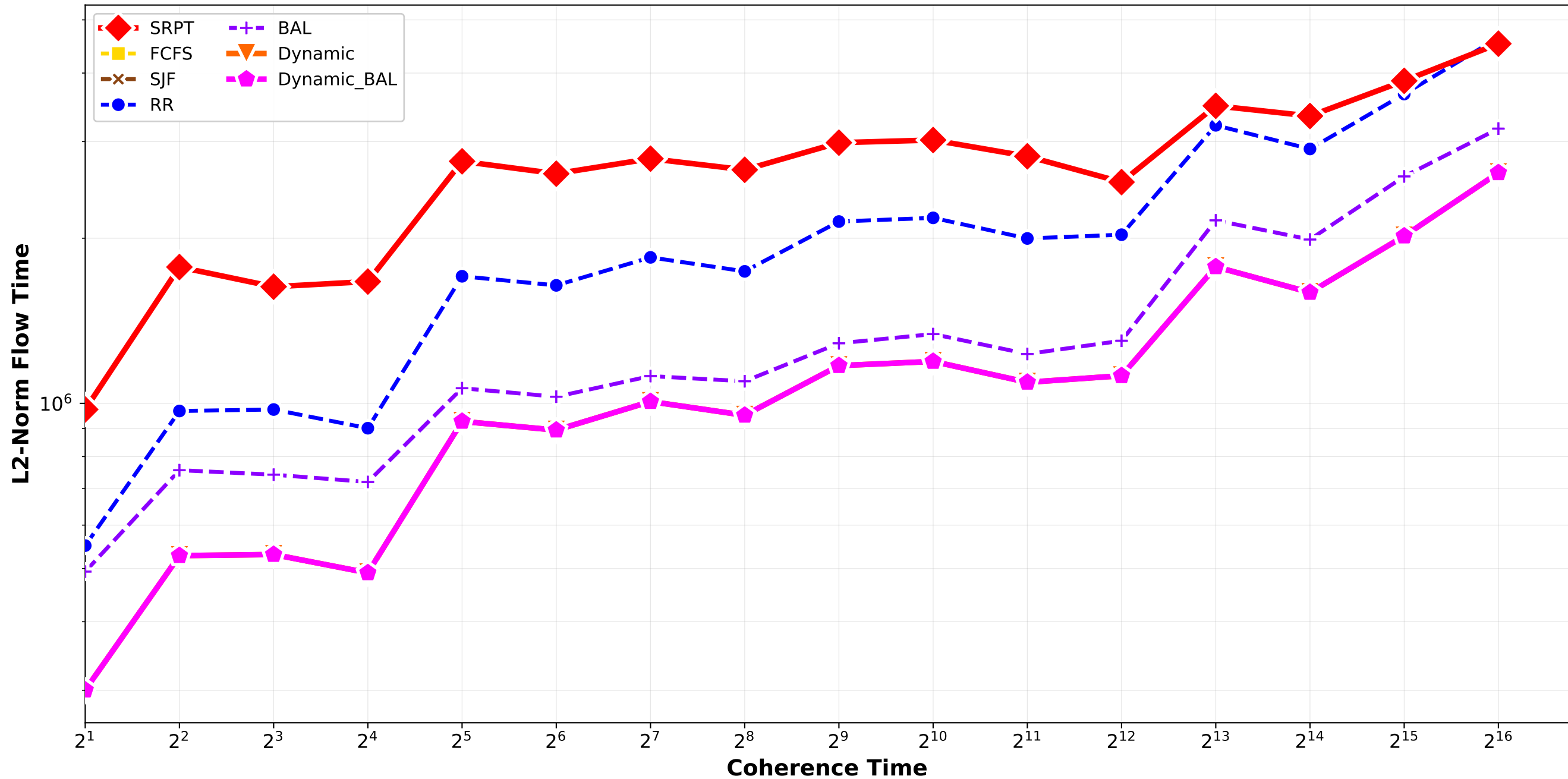
Clairvoyant Algorithms - L2 Norm Flow Time normal_combination_softrandom std6_std9_std12 / triplet_1
