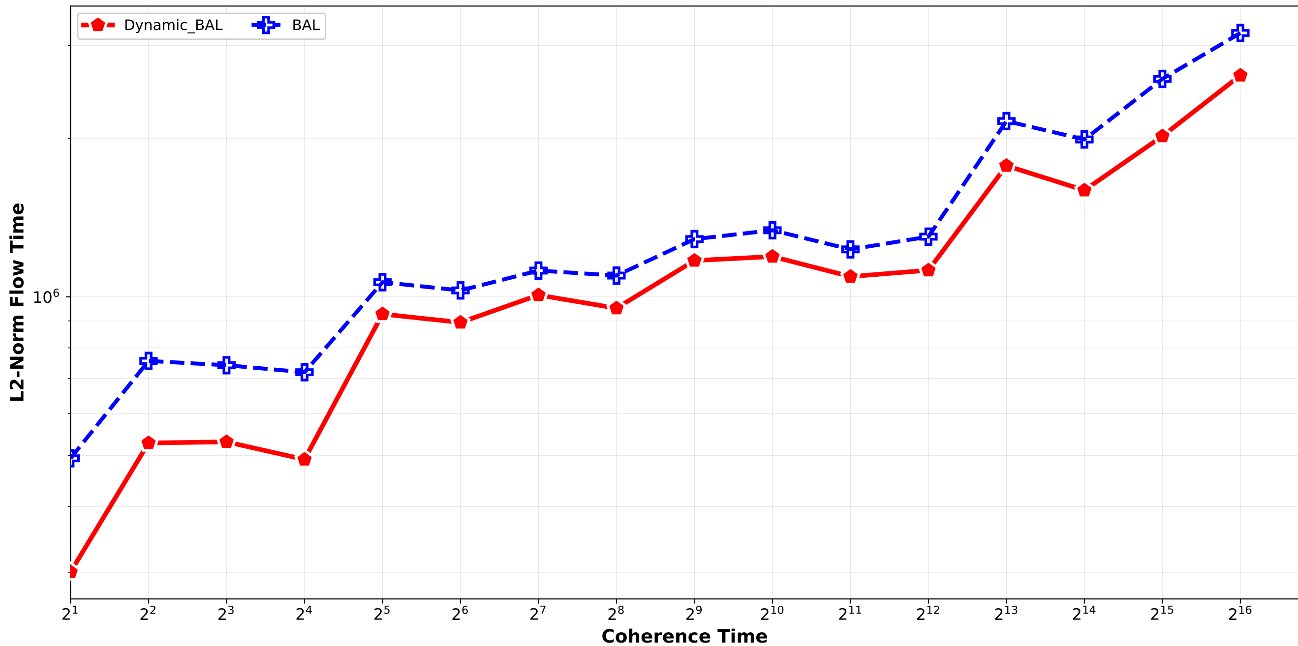
Dynamic_BAL vs BAL - L2 Norm Flow Time normal_combination_software std6_std9_std12 / triplet_1
