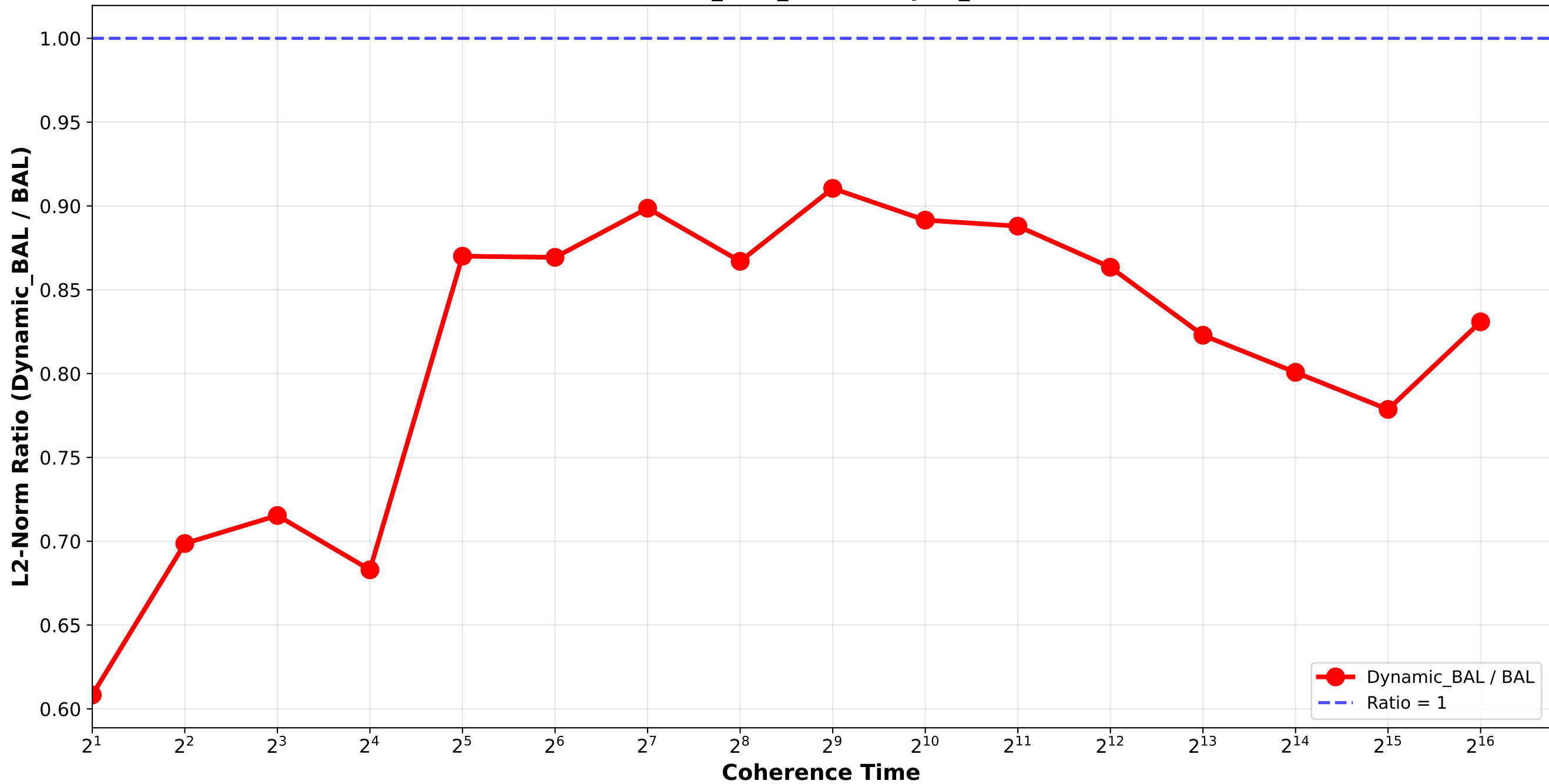
Dynamic_BAL vs BAL - L2 Norm Ratio normal_combination_softrandom std6_std9_std12 / triplet_1
