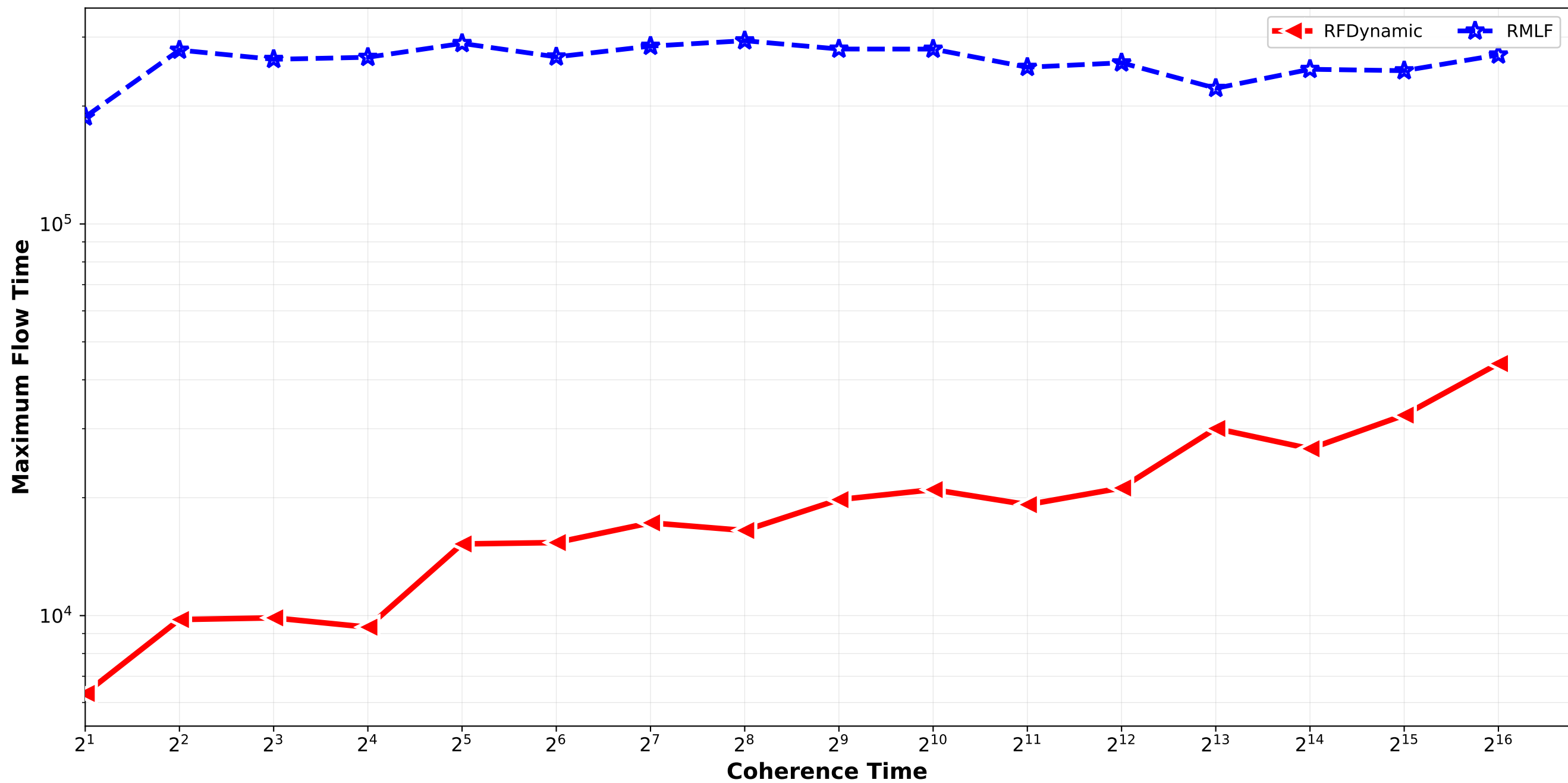
RFDynamic vs RMLF - Maximum Flow Time normal_combination_softrandom std6_std9_std12 / triplet_1
