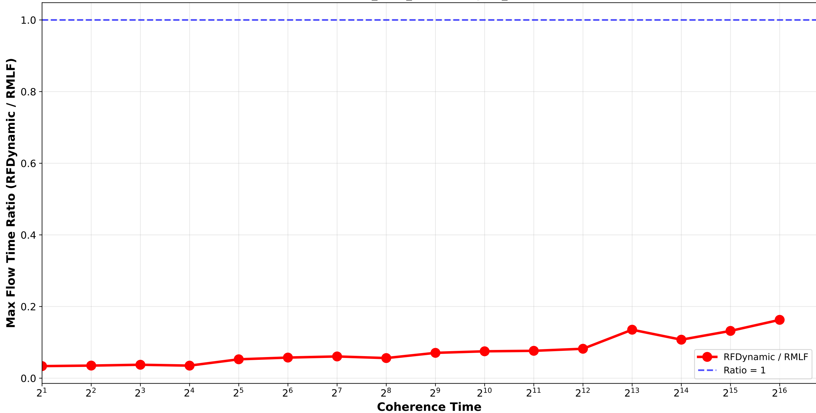
RFDynamic vs RMLF - Max Flow Time Ratio normal_combination_softrandom std6_std9_std12 / triplet_1
