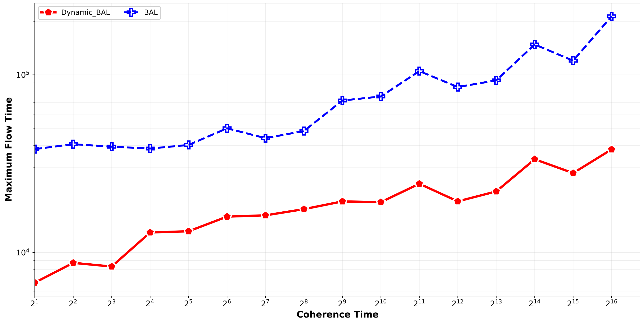
Dynamic_BAL vs BAL - Maximum Flow Time normal_combination_softrandom std9_std12_std15 / triplet_2
