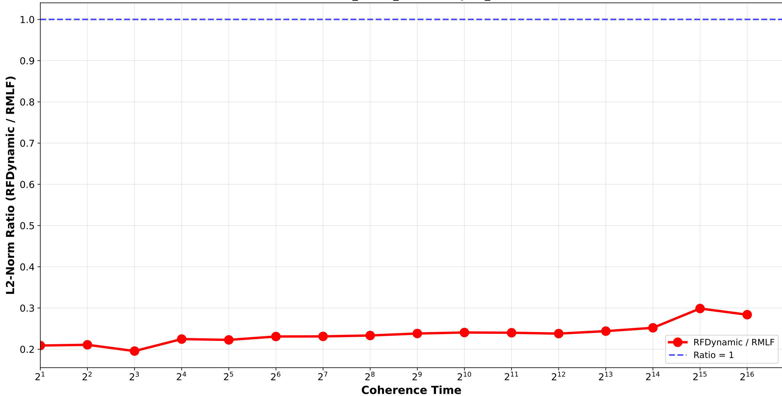
RFDynamic vs RMLF - L2 Norm Ratio normal_combination_softrandom std9_std12_std15 / triplet_2
