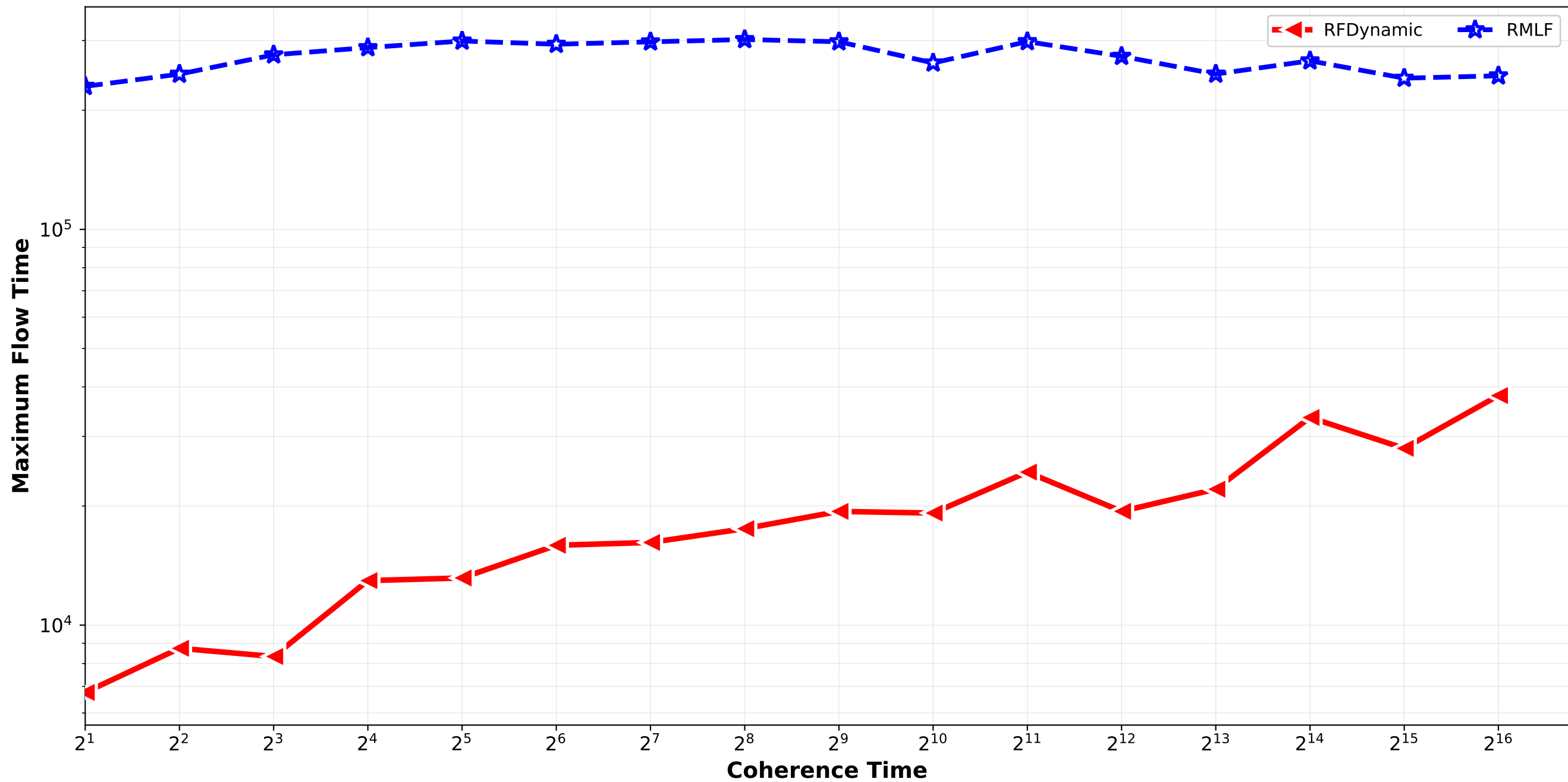
RFDynamic vs RMLF - Maximum Flow Time normal_combination_softrandom std9_std12_std15 / triplet_2
