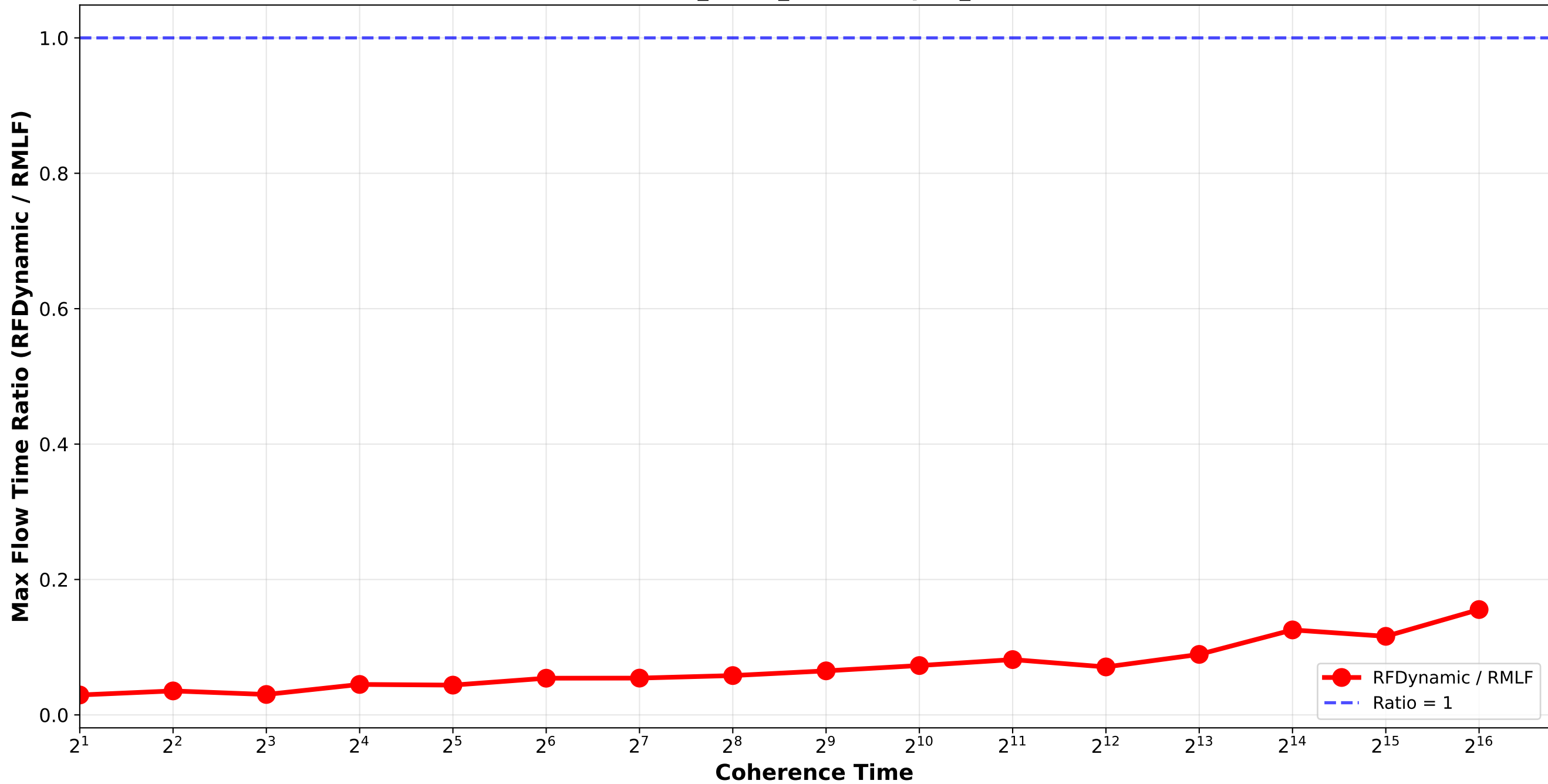
RFDynamic vs RMLF - Max Flow Time Ratio normal_combination_softrandom std9_std12_std15 / triplet_2
