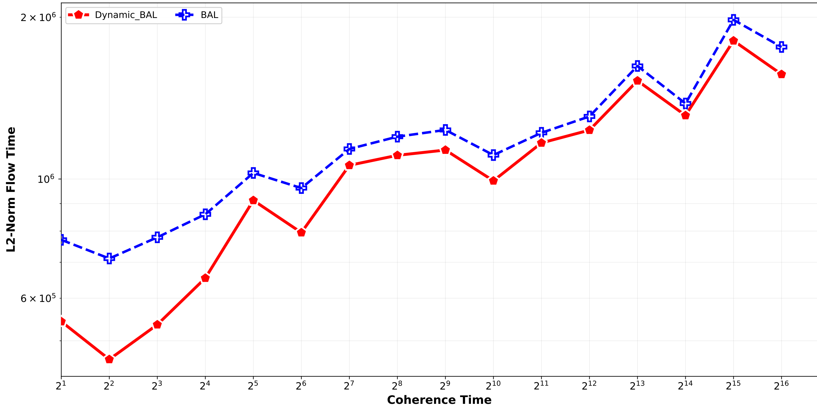
Dynamic_BAL vs BAL - L2 Norm Flow Time normal_combination_softrandom std12_std15 / pair_3
