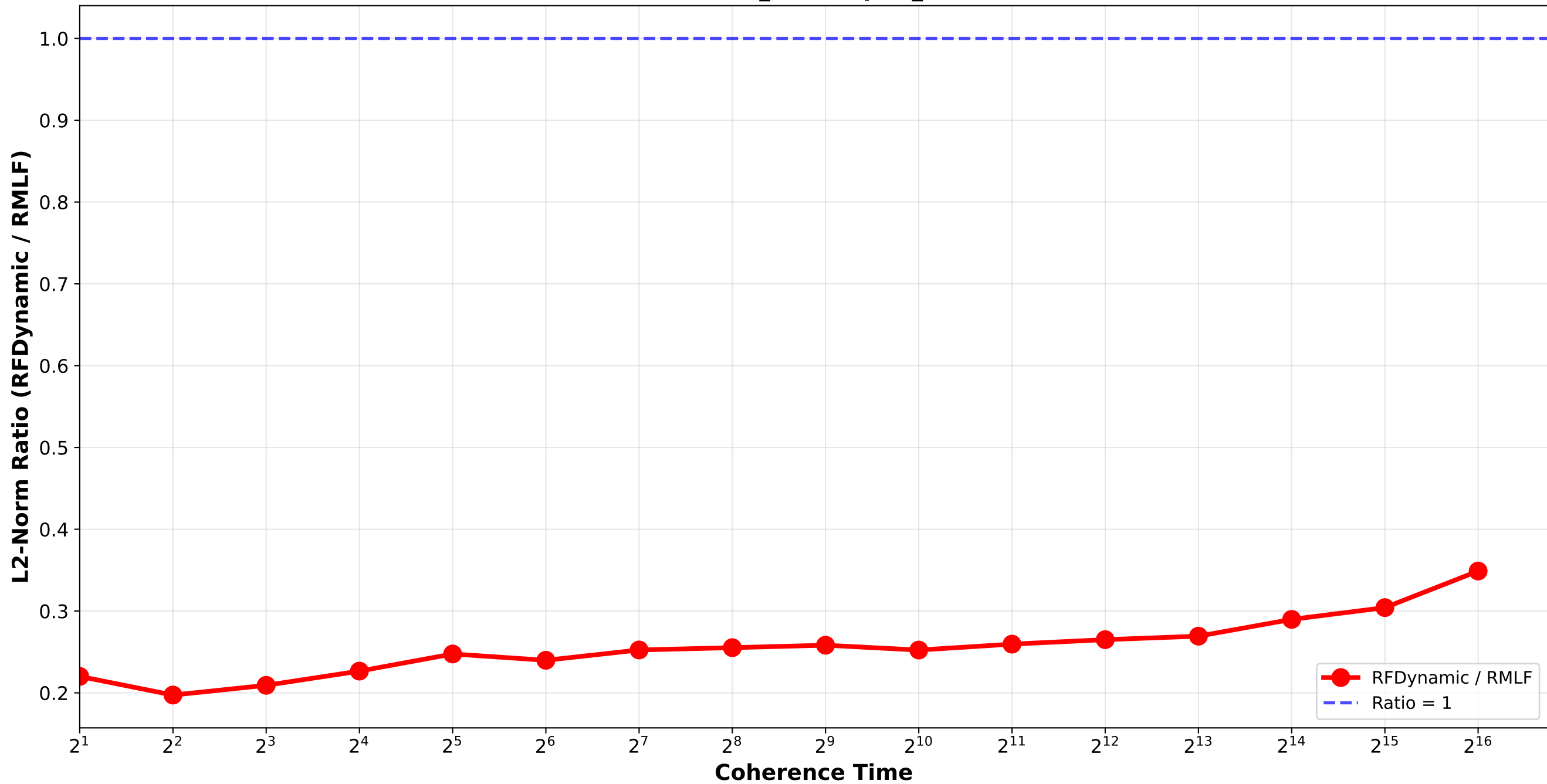
RFDynamic vs RMLF - L2 Norm Ratio normal_combination_softrandom std12_std15 / pair_3
