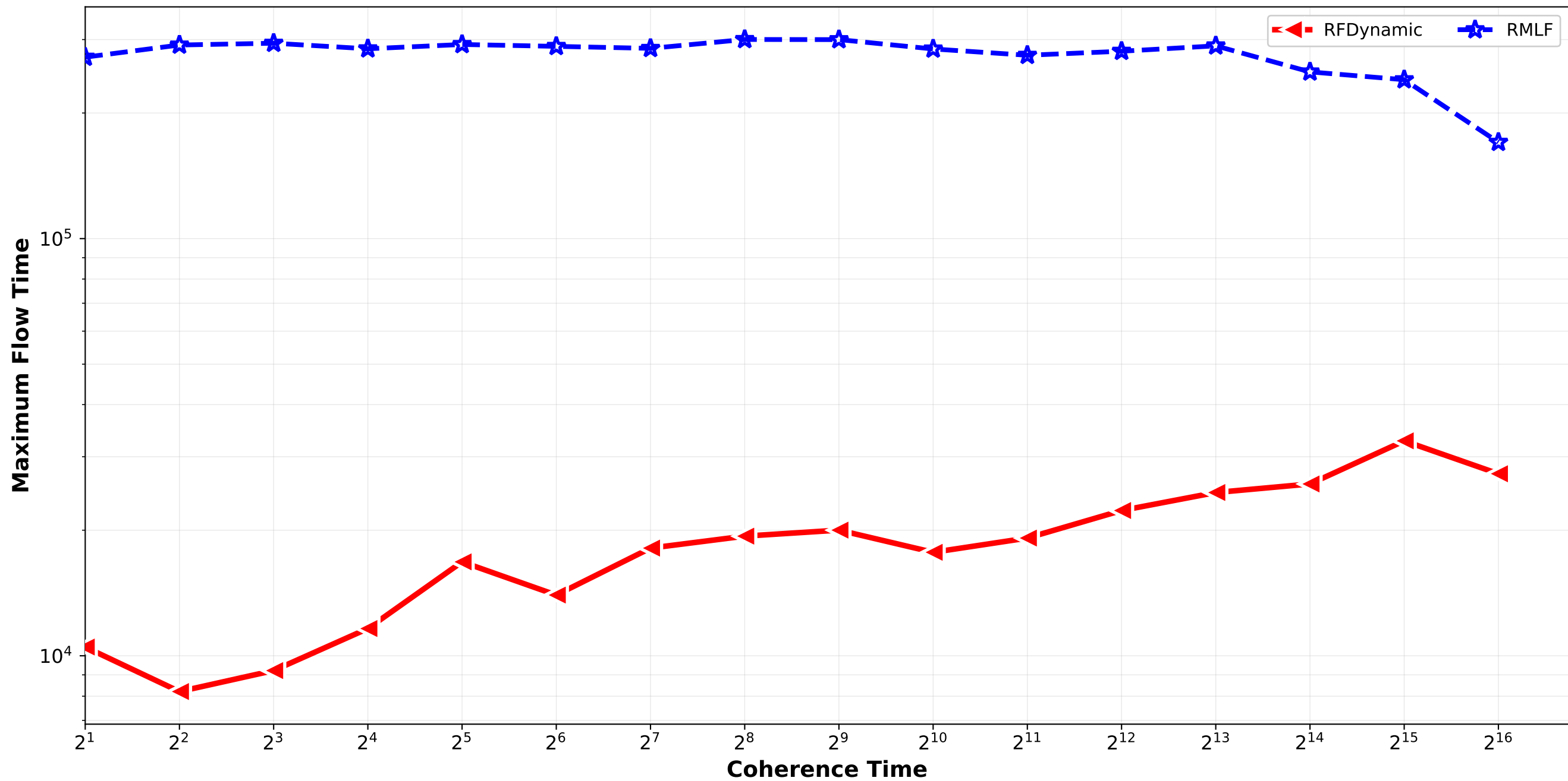
RFDynamic vs RMLF - Maximum Flow Time normal_combination_softrandom std12_std15 / pair_3
