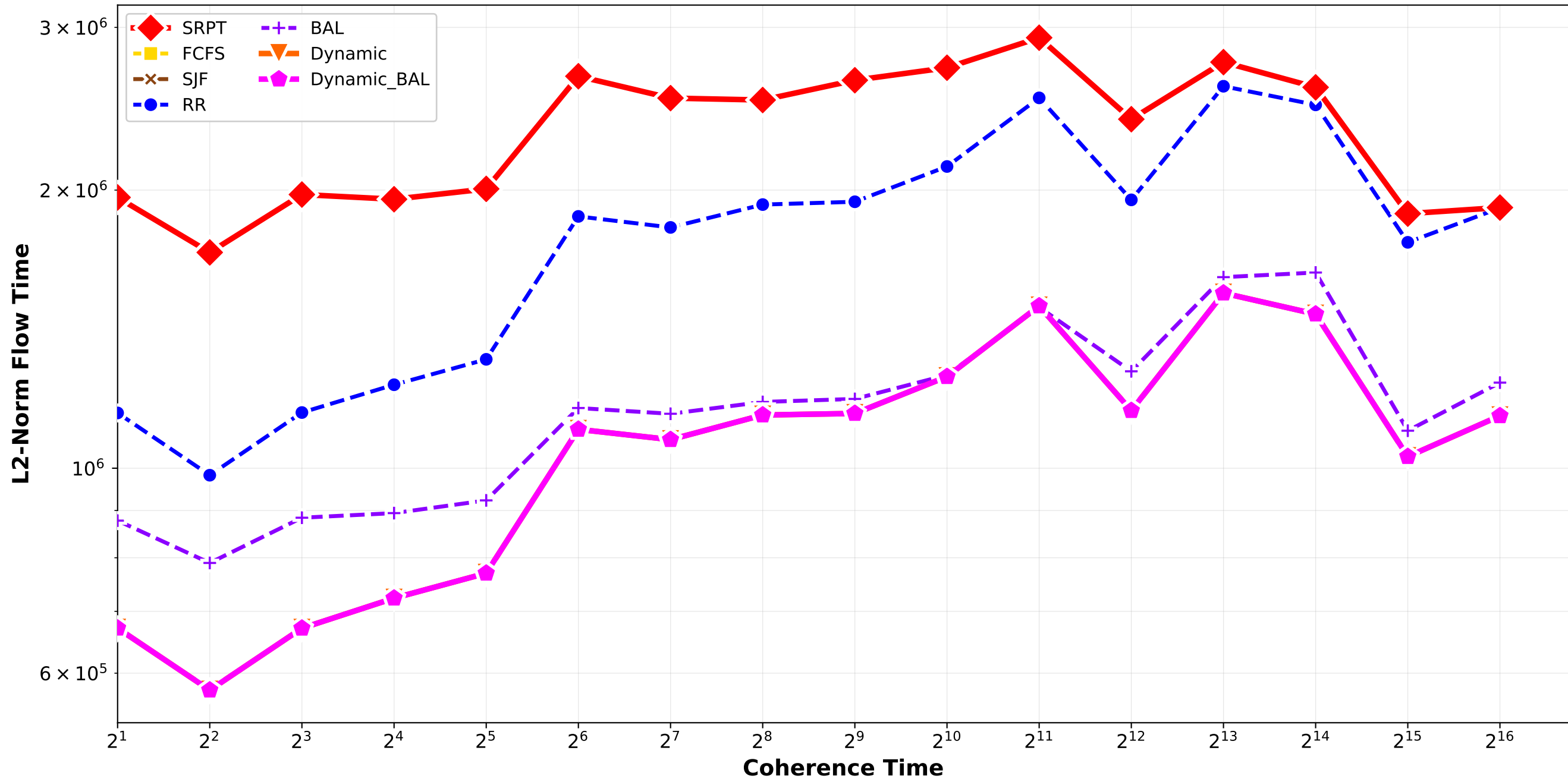
Clairvoyant Algorithms - L2 Norm Flow Time normal_combination_softrandom std15_std18 / pair_4
