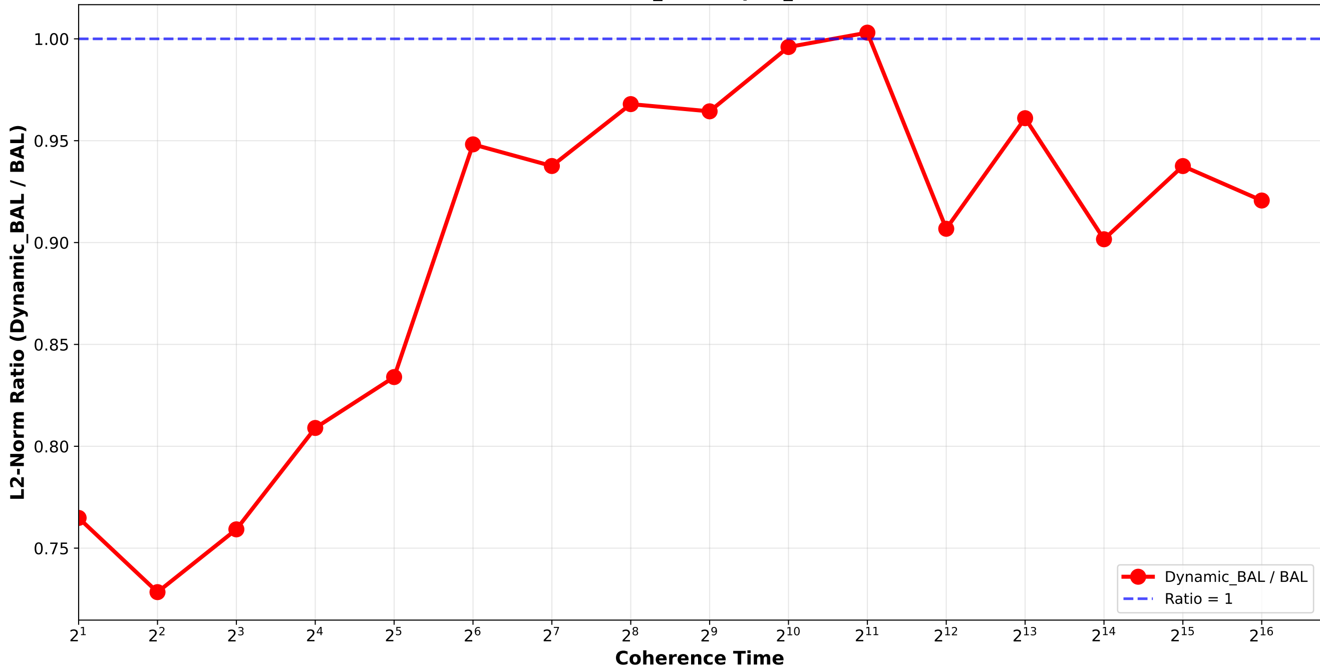
Dynamic_BAL vs BAL - L2 Norm Ratio normal_combination_softrandom std15_std18 / pair_4
