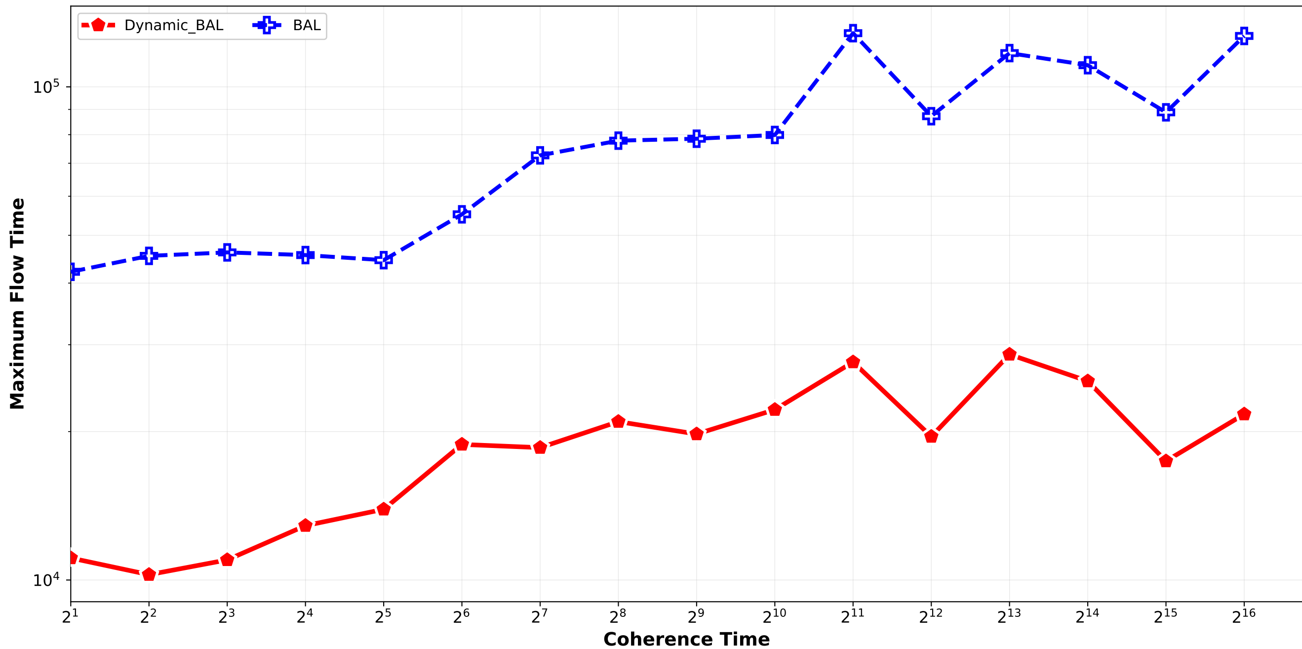
Dynamic_BAL vs BAL - Maximum Flow Time normal_combination_softrandom std15_std18 / pair_4
