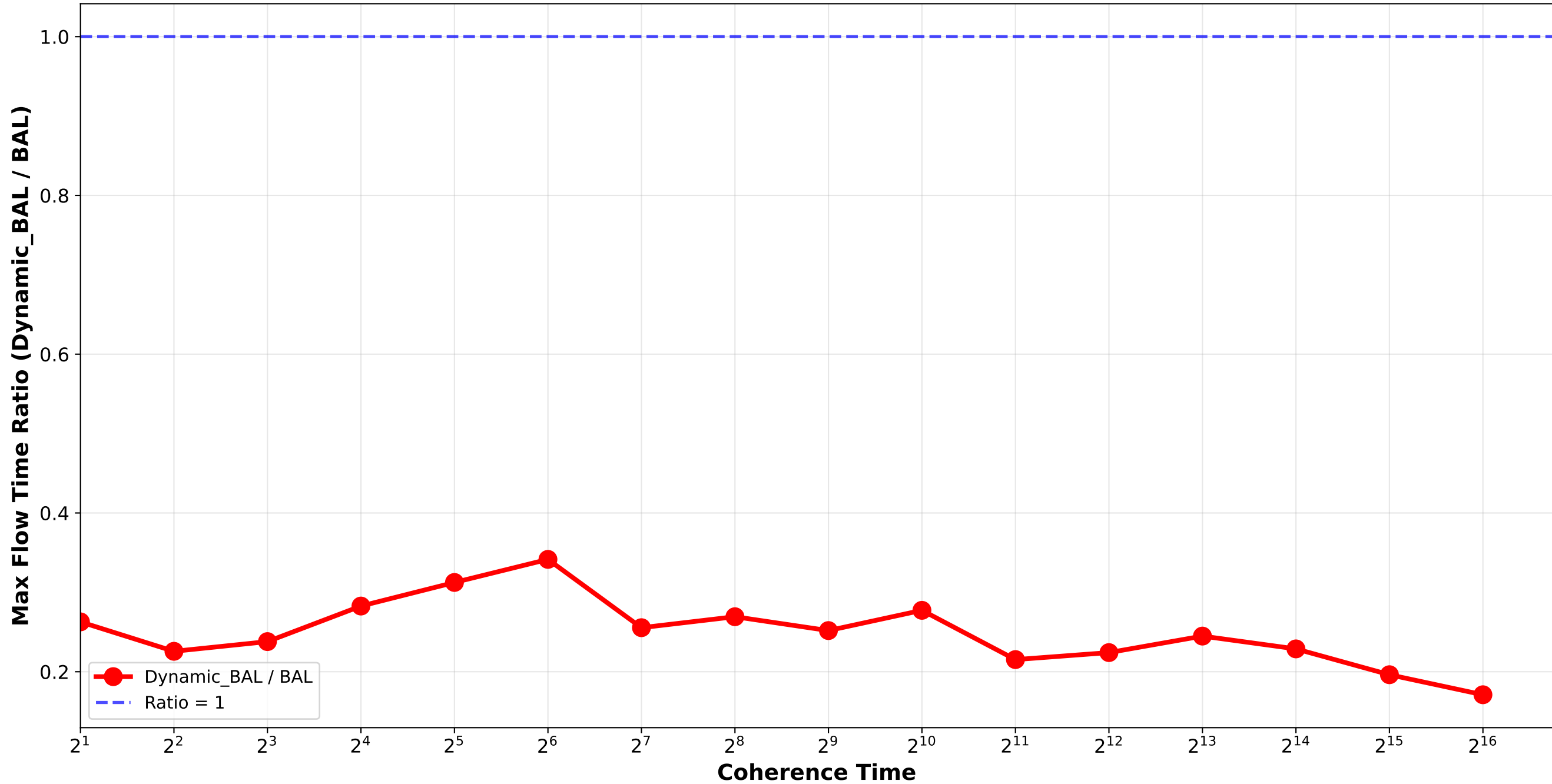
Dynamic_BAL vs BAL - Max Flow Time Ratio normal_combination_softrandom std15_std18 / pair_4
