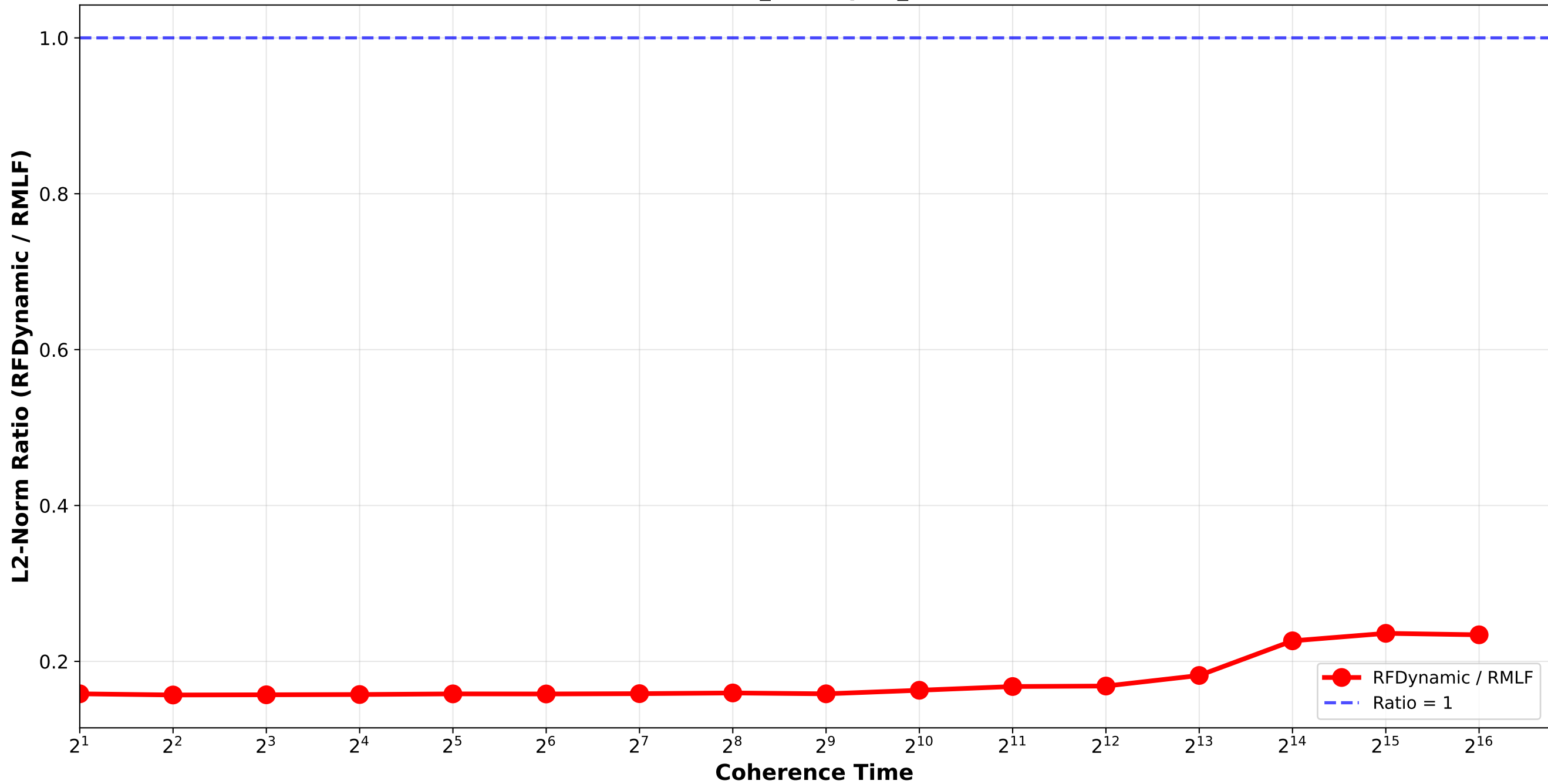
RFDynamic vs RMLF - L2 Norm Ratio normal_combination_softrandom std6_std9 / pair_1
