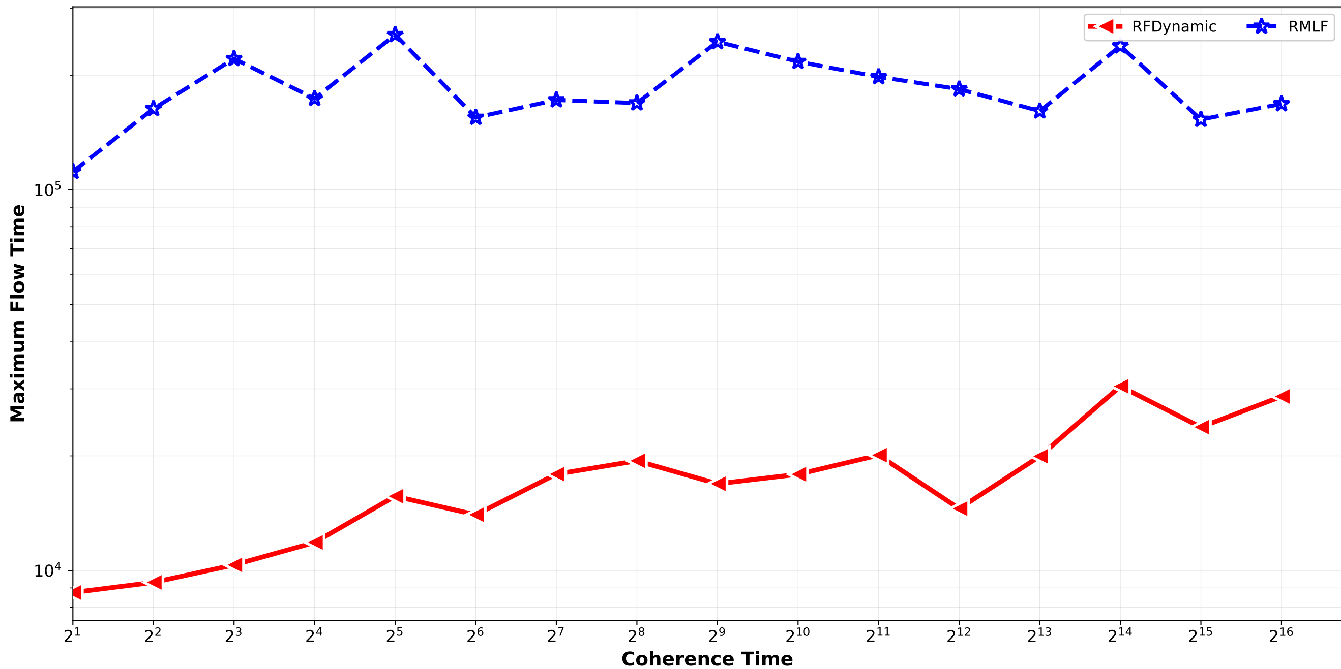
RFDynamic vs RMLF - Maximum Flow Time normal_combination_softrandom std6_std9 / pair_1
