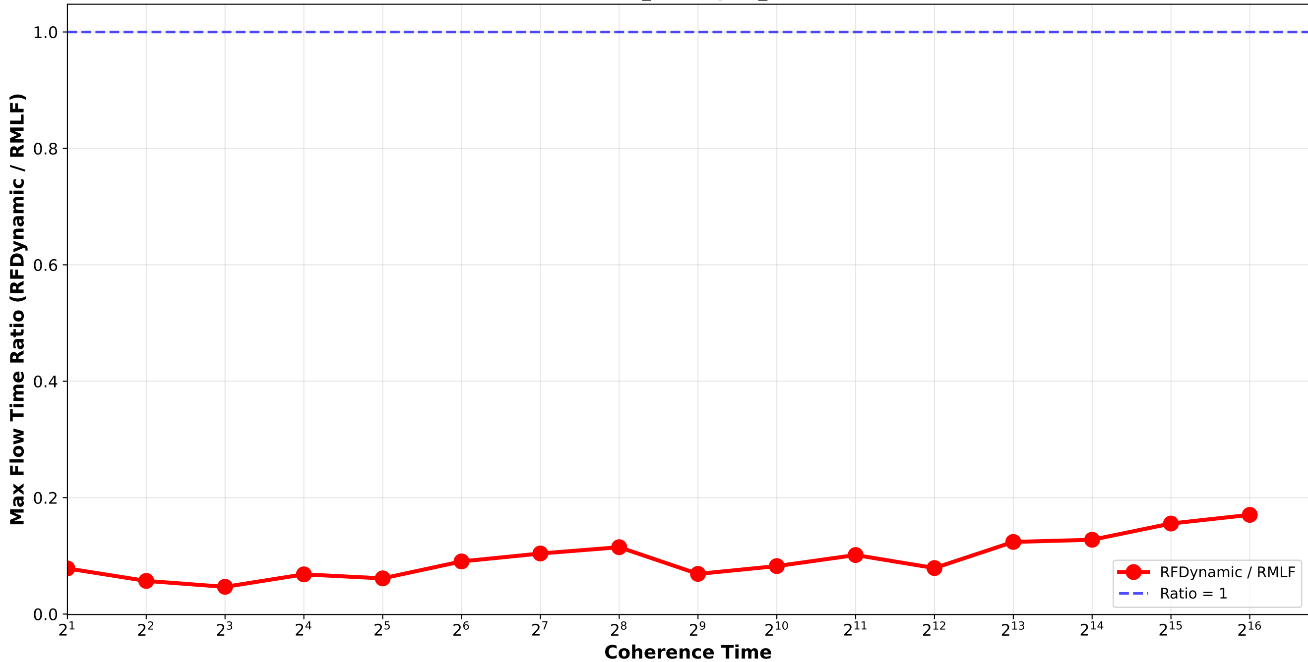
RFDynamic vs RMLF - Max Flow Time Ratio normal_combination_softrandom std6_std9 / pair_1
