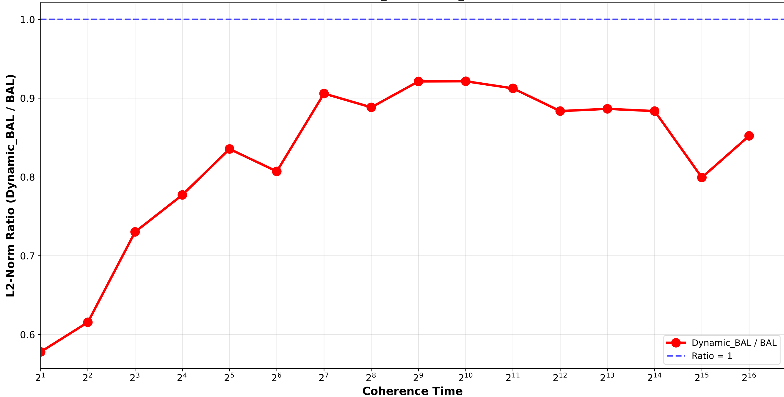
Dynamic_BAL vs BAL - L2 Norm Ratio normal_combination_softrandom std9_std12 / pair_2
