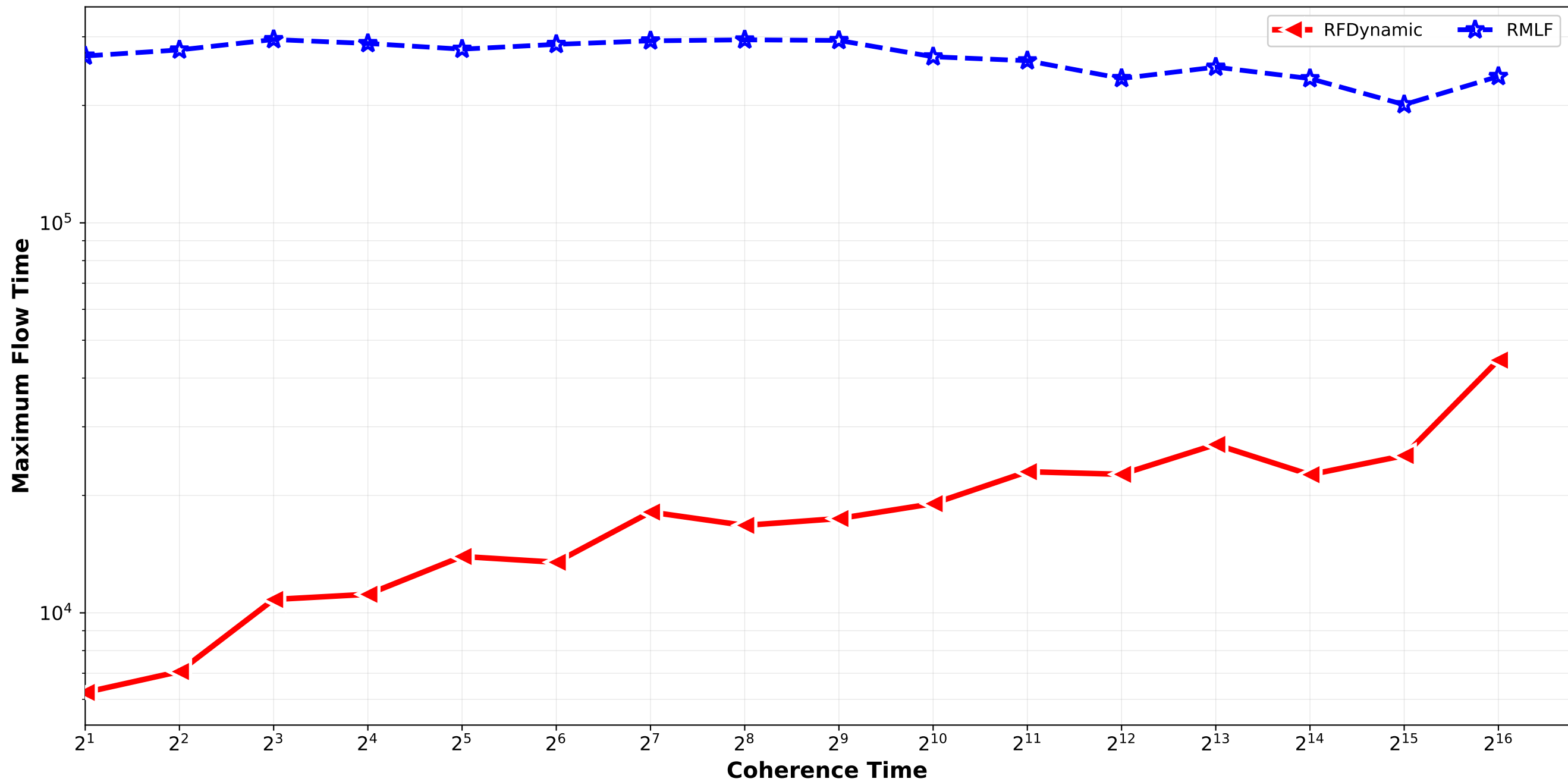
RFDynamic vs RMLF - Maximum Flow Time normal_combination_softrandom std9_std12 / pair_2
