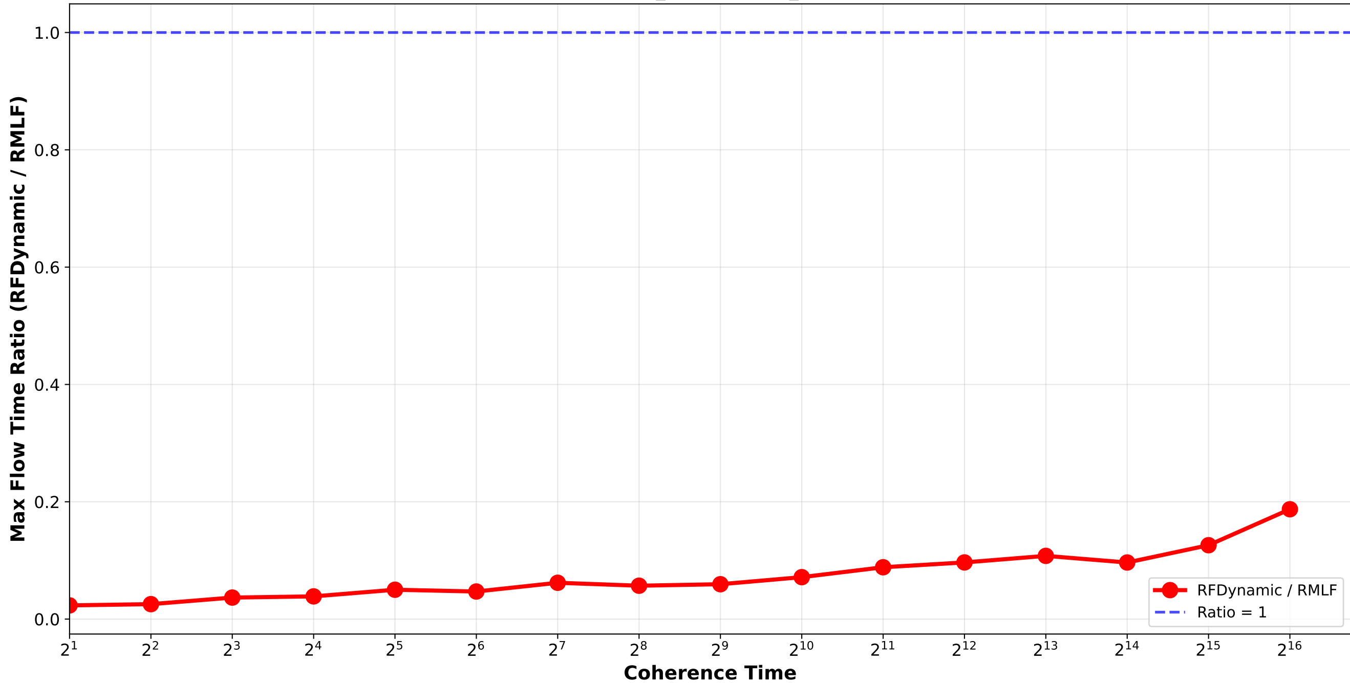
RFDynamic vs RMLF - Max Flow Time Ratio normal_combination_softrandom std9_std12 / pair_2
