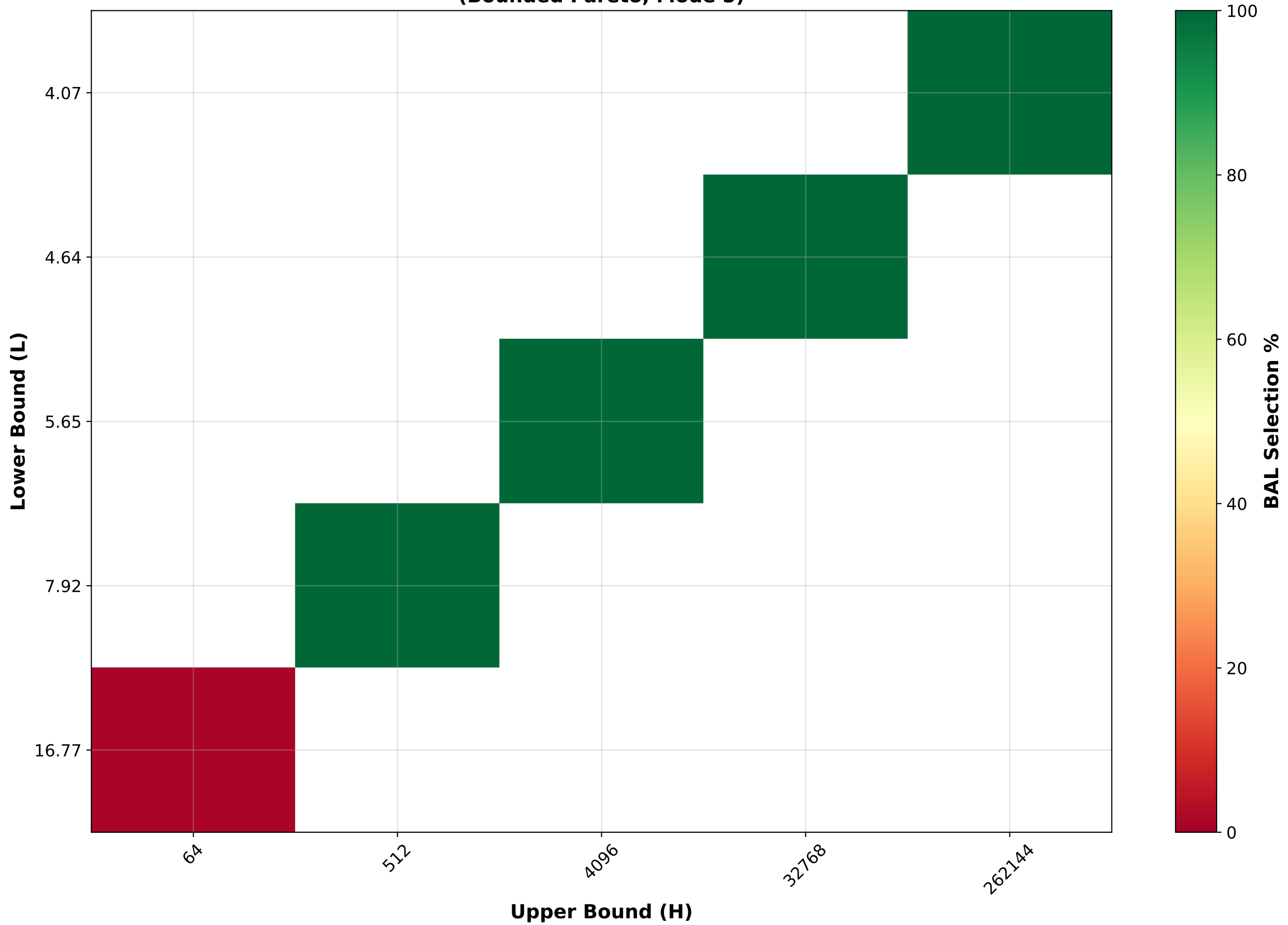
Dynamic_BAL: BAL Selection Percentage Heatmap (Bounded Pareto, Mode 5)
