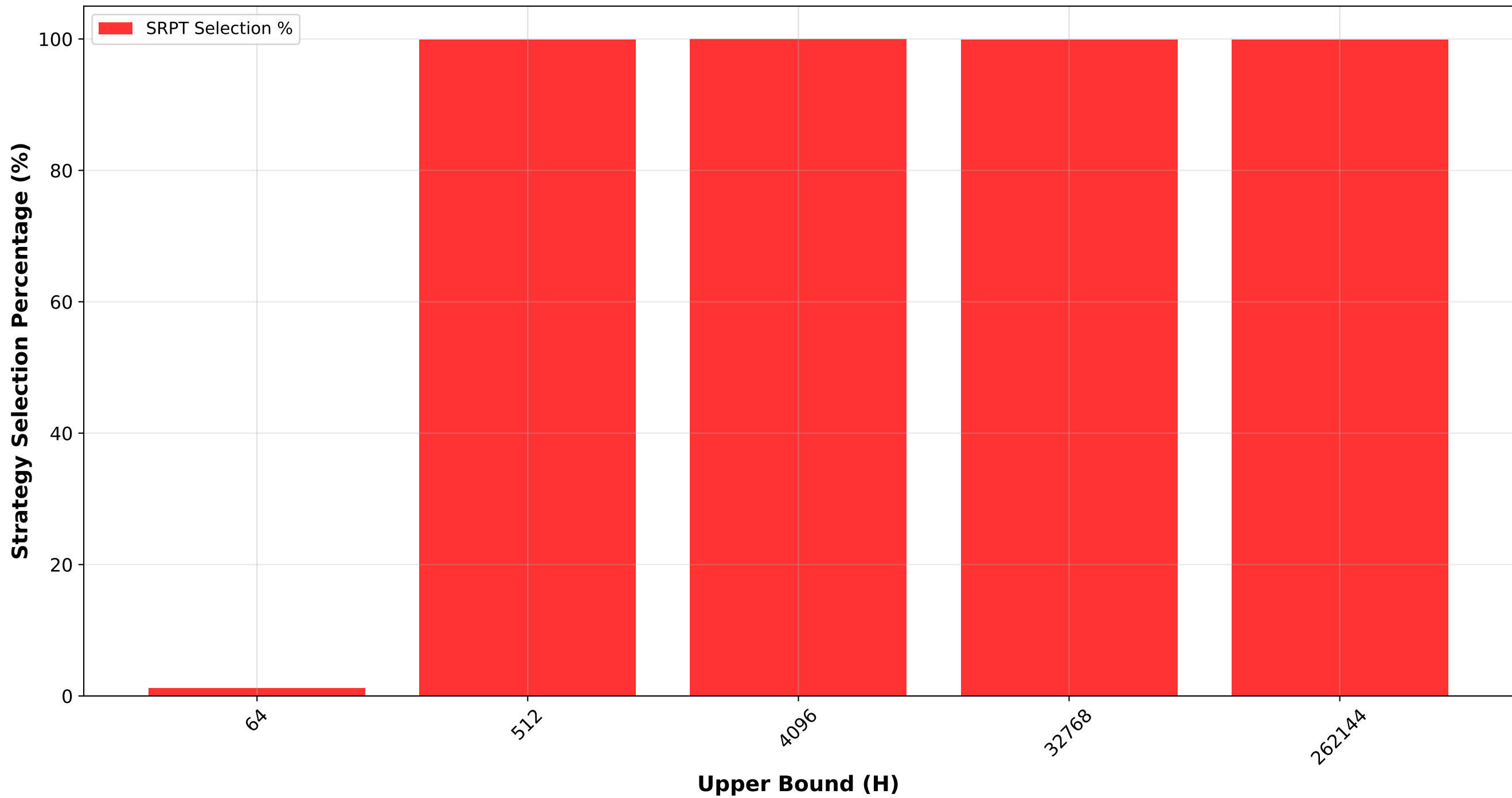
Dynamic: SRPT vs FCFS Selection Rate (Bounded Pareto Distribution, Mode 5)
