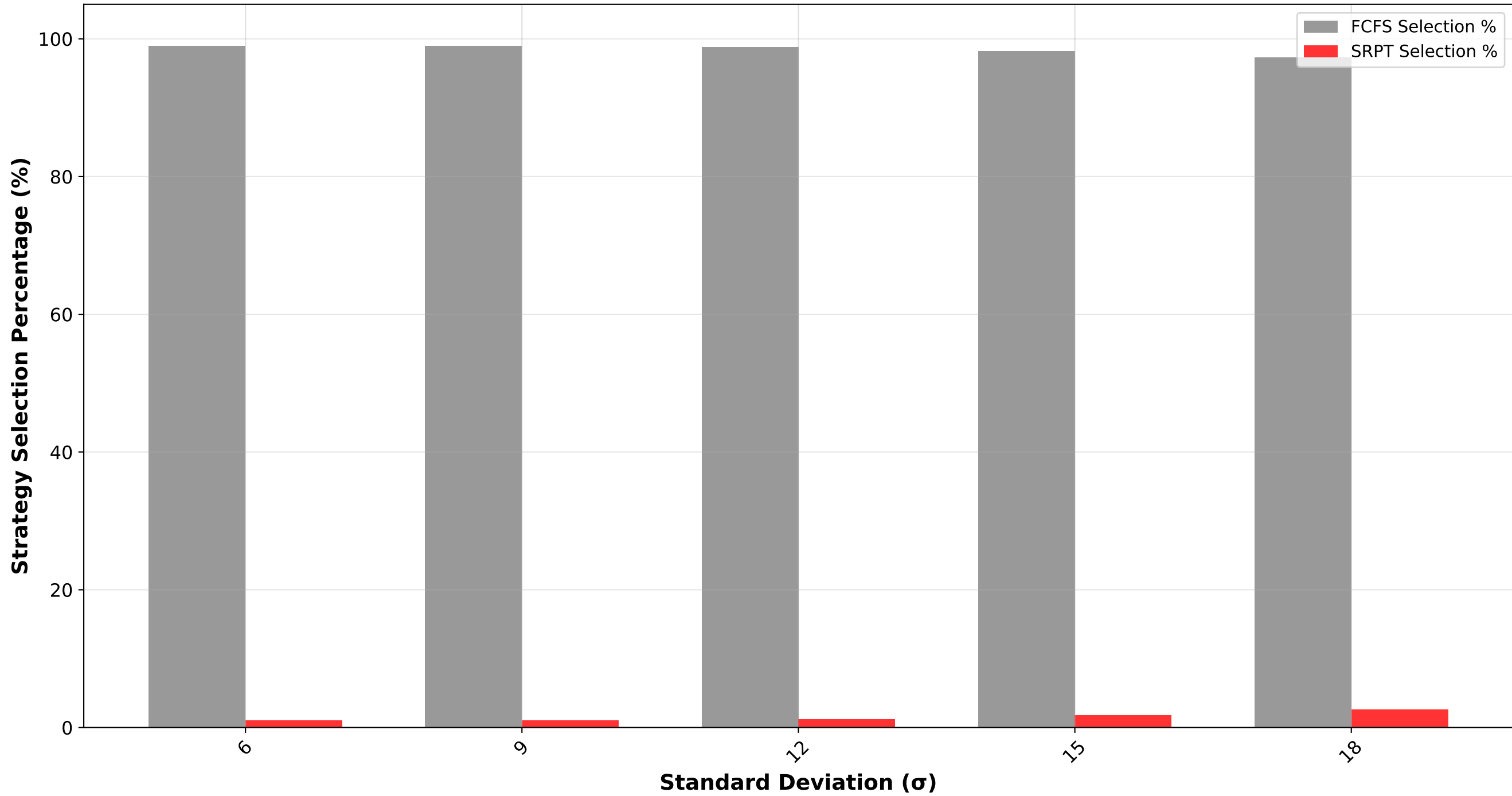
Dynamic: SRPT vs FCFS Selection Rate (Normal Distribution, Mode 5)
