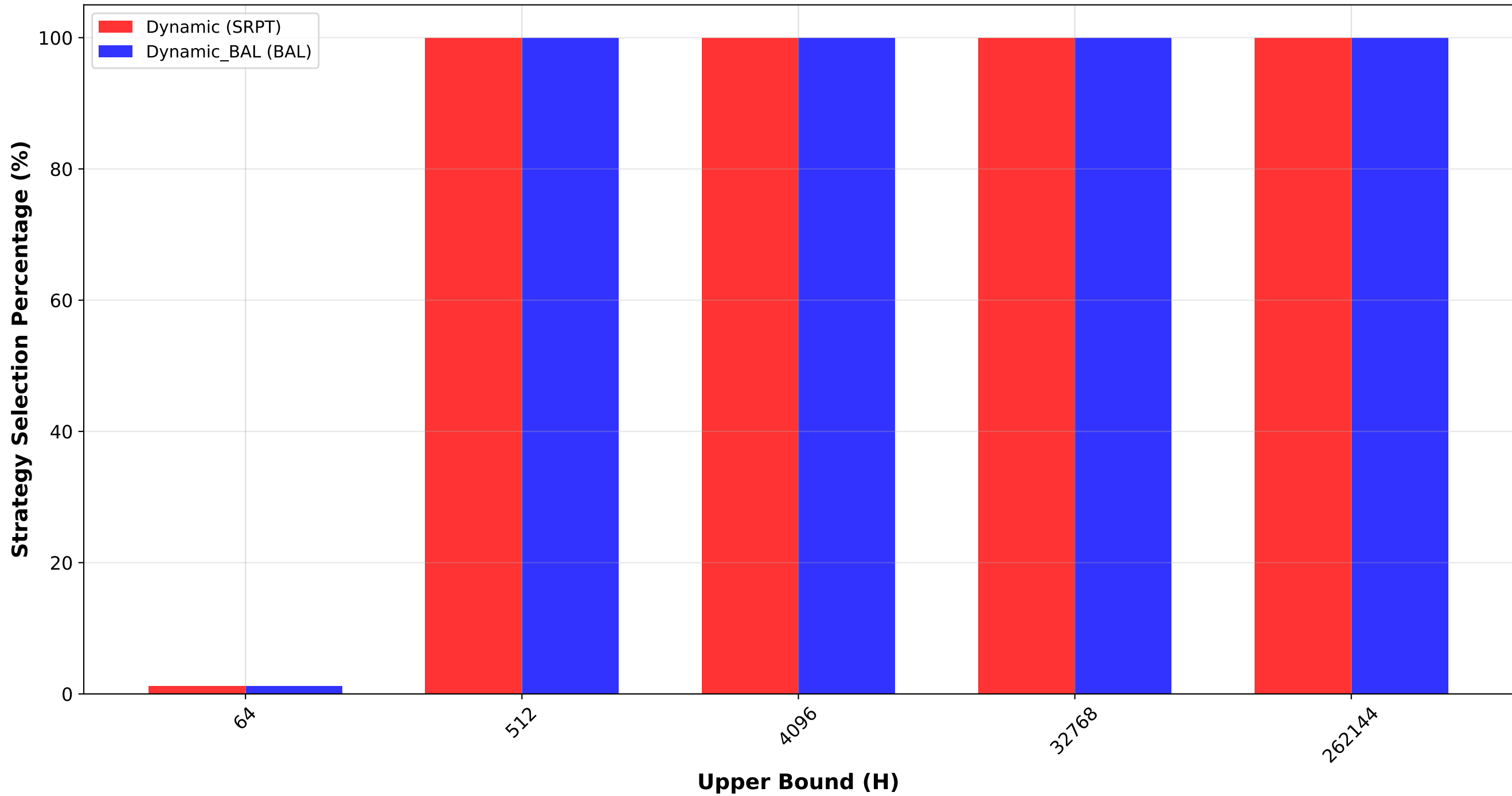
Dynamic vs Dynamic_BAL: Strategy Selection Comparison (Bounded Pareto, Mode 5)
