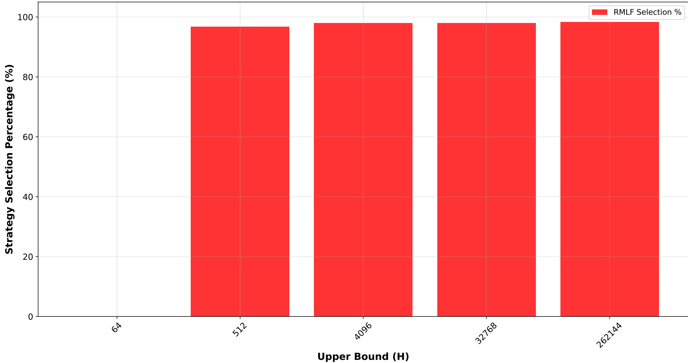
RFDynamic: RMLF vs FCFS Selection Rate (Bounded Pareto Distribution, Mode 5)
