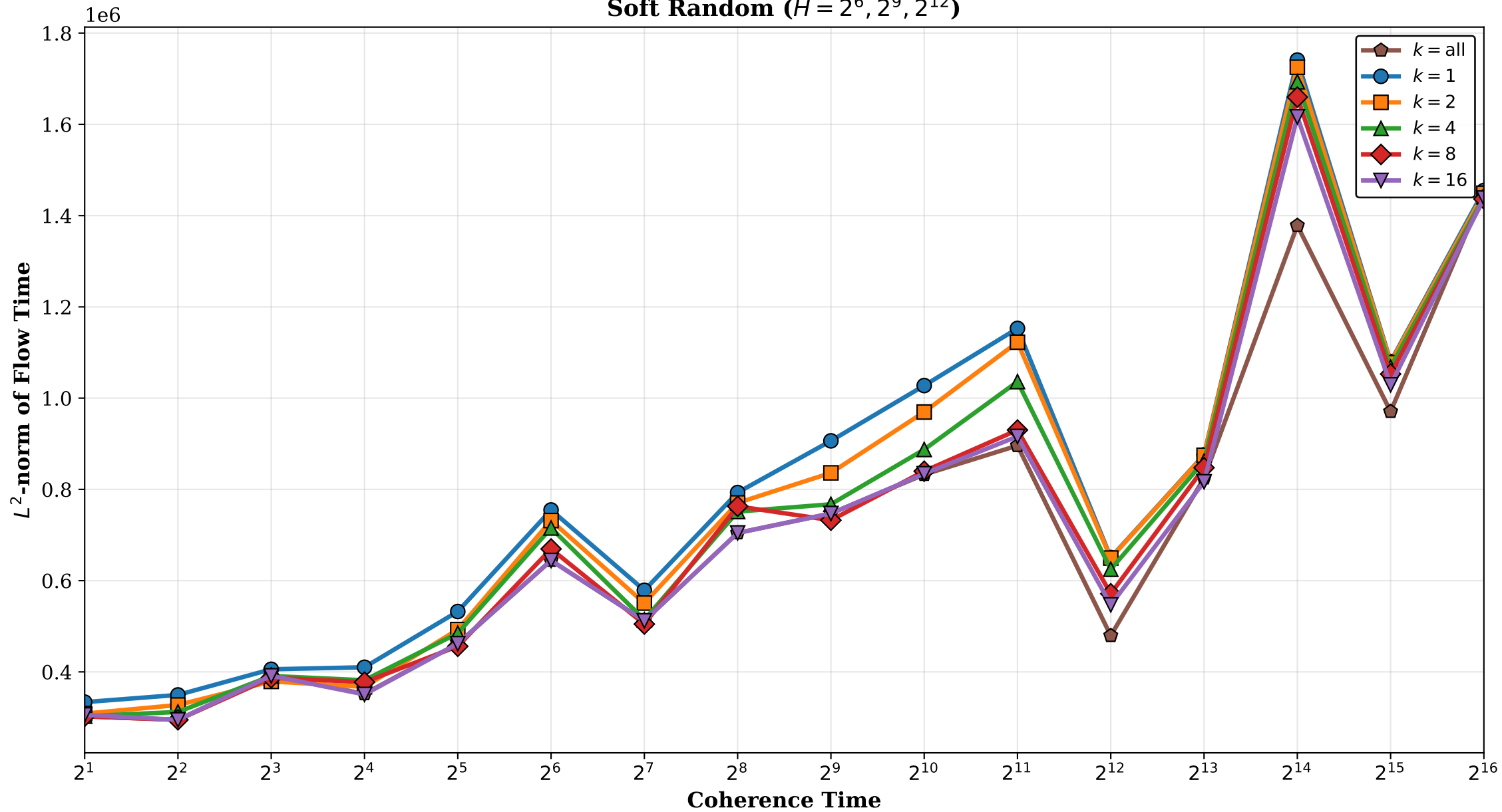
Dynamic Lookback Comparison Soft Random ( H = 2^6, 2^9, 2^{12} )
