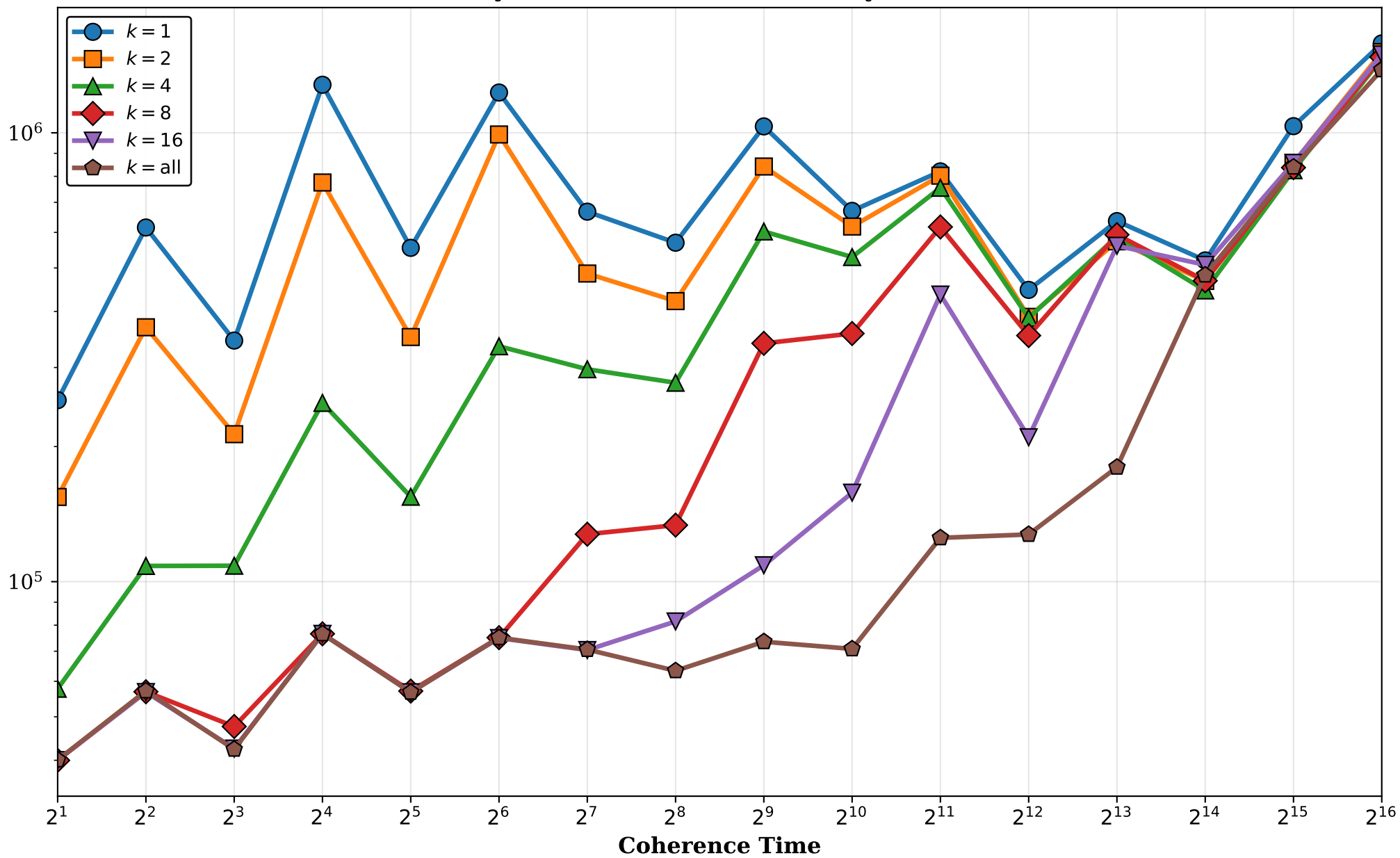
RFDynamic Lookback Sensitivity ( B = 100 )
