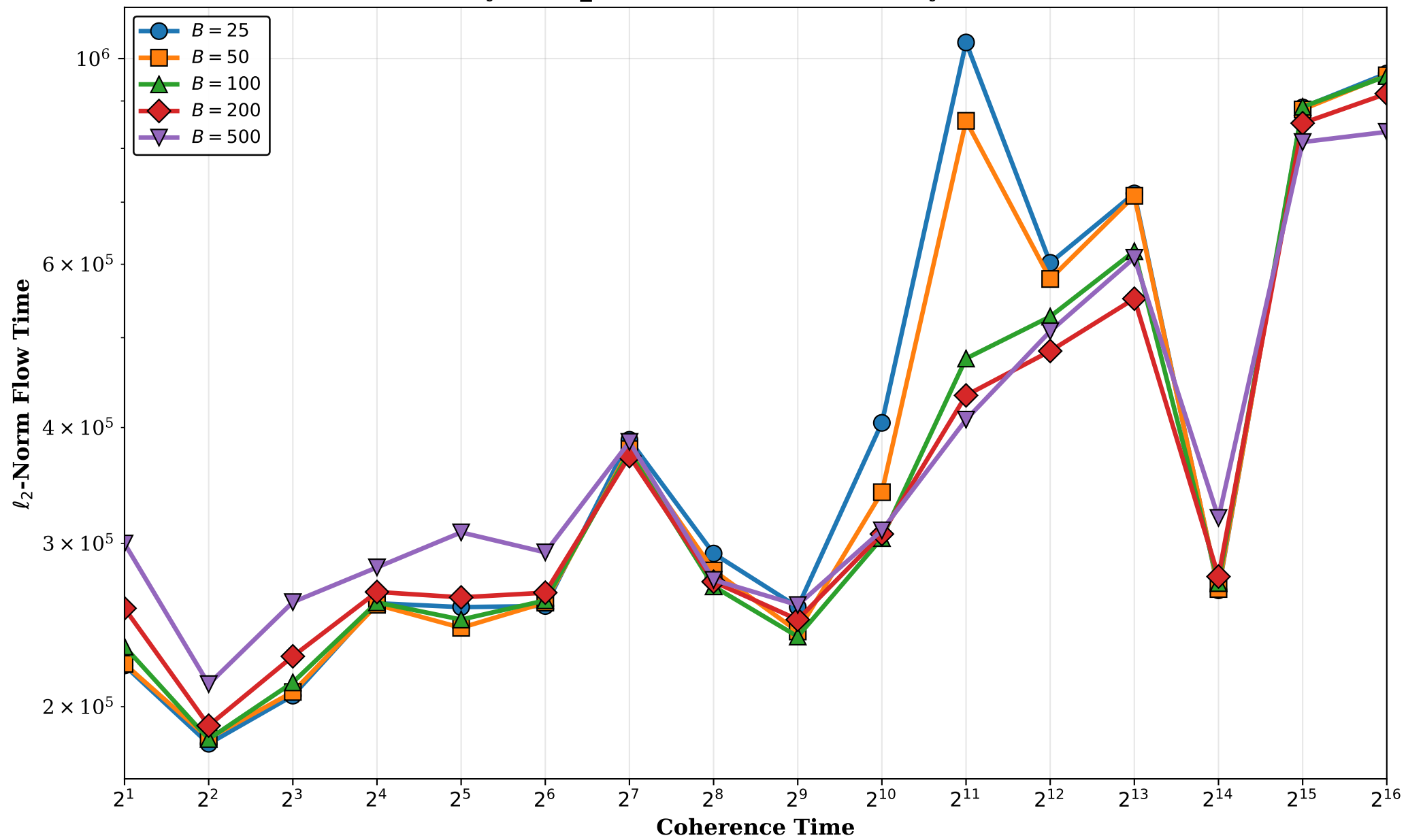
Dynamic_BAL Batch Size Sensitivity ( k = 16 )
