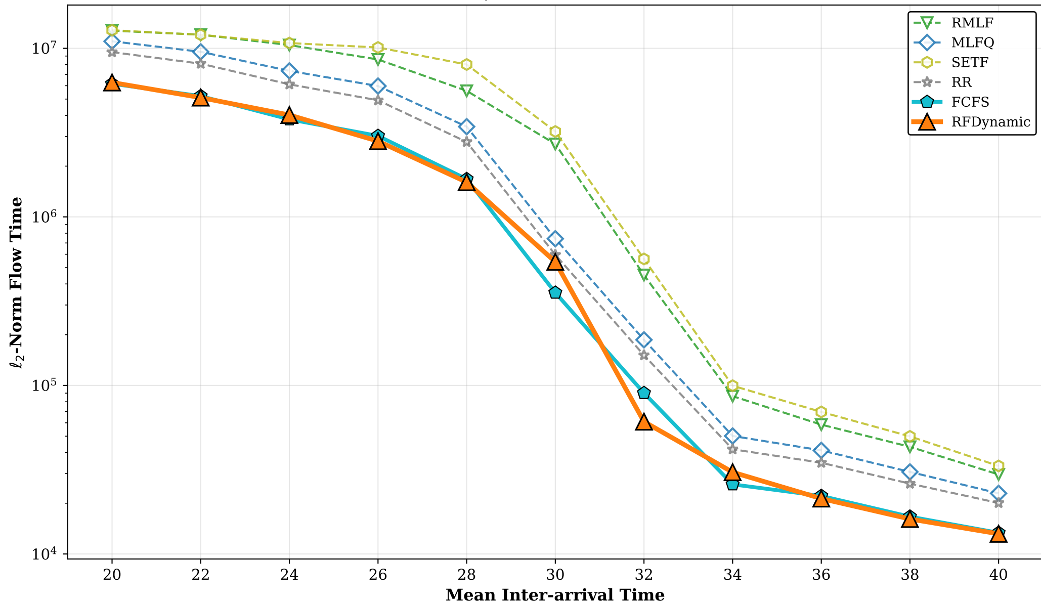
Non-Clairvoyant \ell_2 -Norm Comparison Normal ( \mu = 30, \sigma = 18, CV=0.60 )
