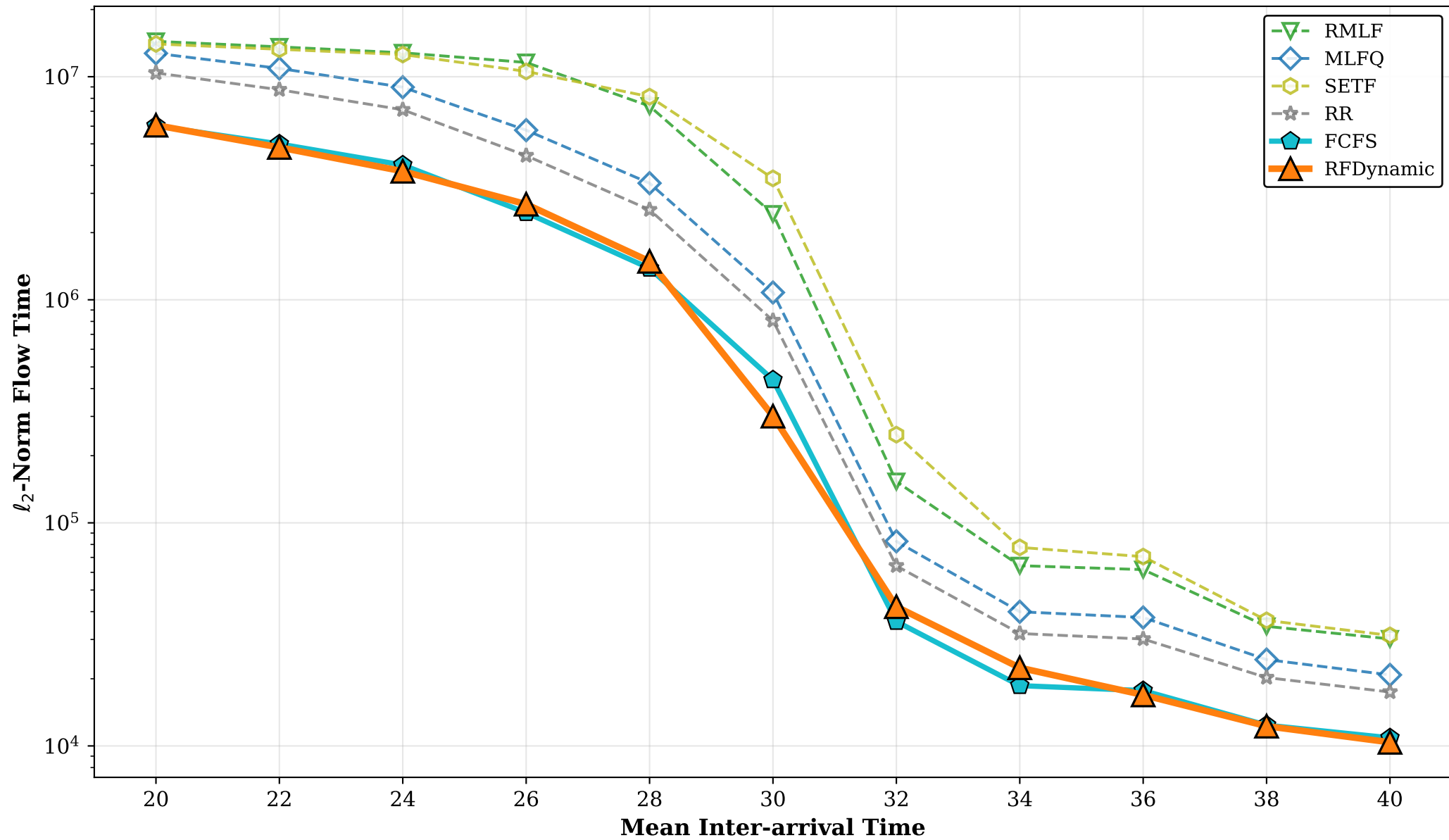
Non-Clairvoyant \ell_2 -Norm Comparison Normal ( \mu = 30, \sigma = 9, CV=0.30 )
