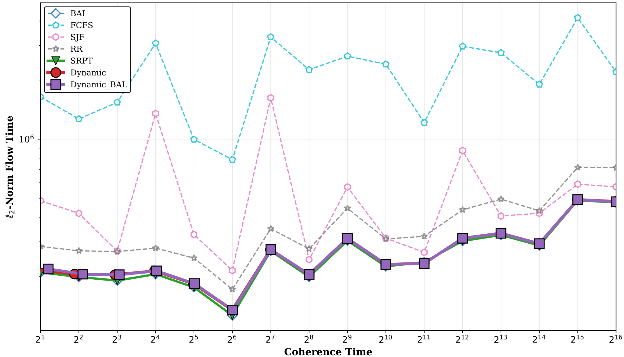
Clairvoyant \ell_2 -Norm Comparison Soft Random ( H = 2^{12}, 2^{15}, 2^{18} )
