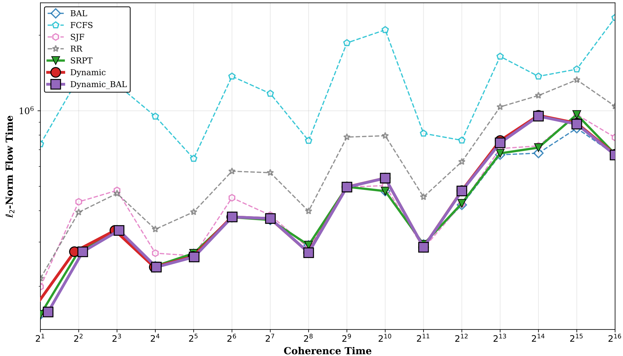
Clairvoyant \ell_2 -Norm Comparison Soft Random ( H = 2^6, 2^9, 2^{12}, 2^{15} )
