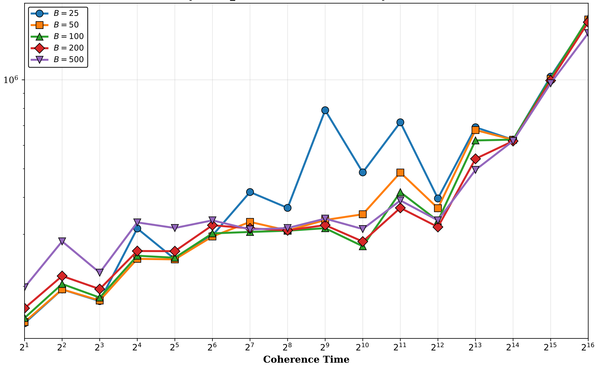
Dynamic_BAL Batch Size Sensitivity ( k = 16 )
