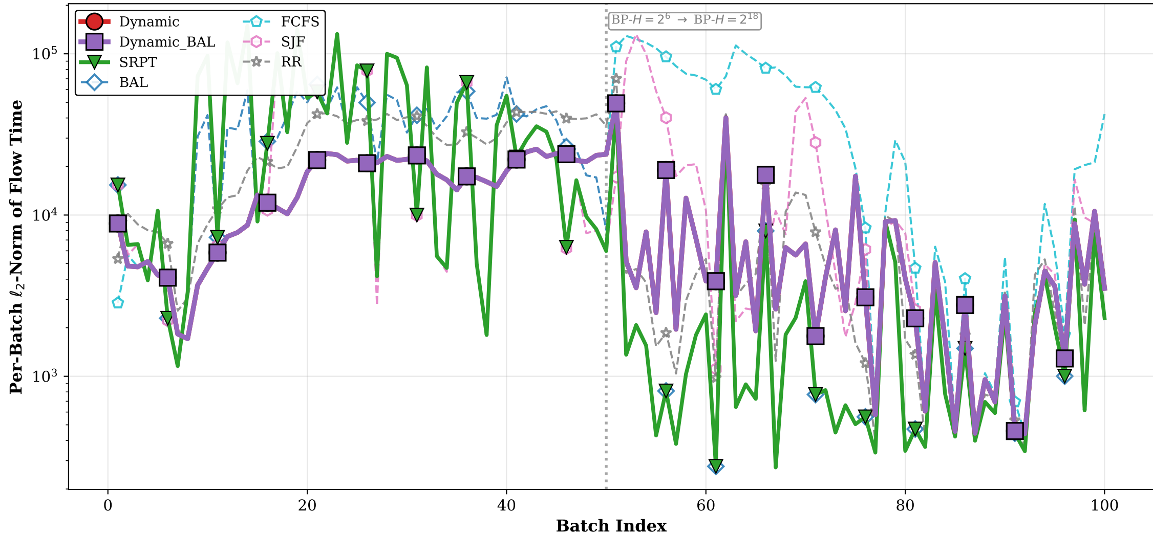
Clairvoyant: Distribution Shift ( \text{BP-H} = 2^6 \rightarrow \text{BP-H} = 2^{18} )
