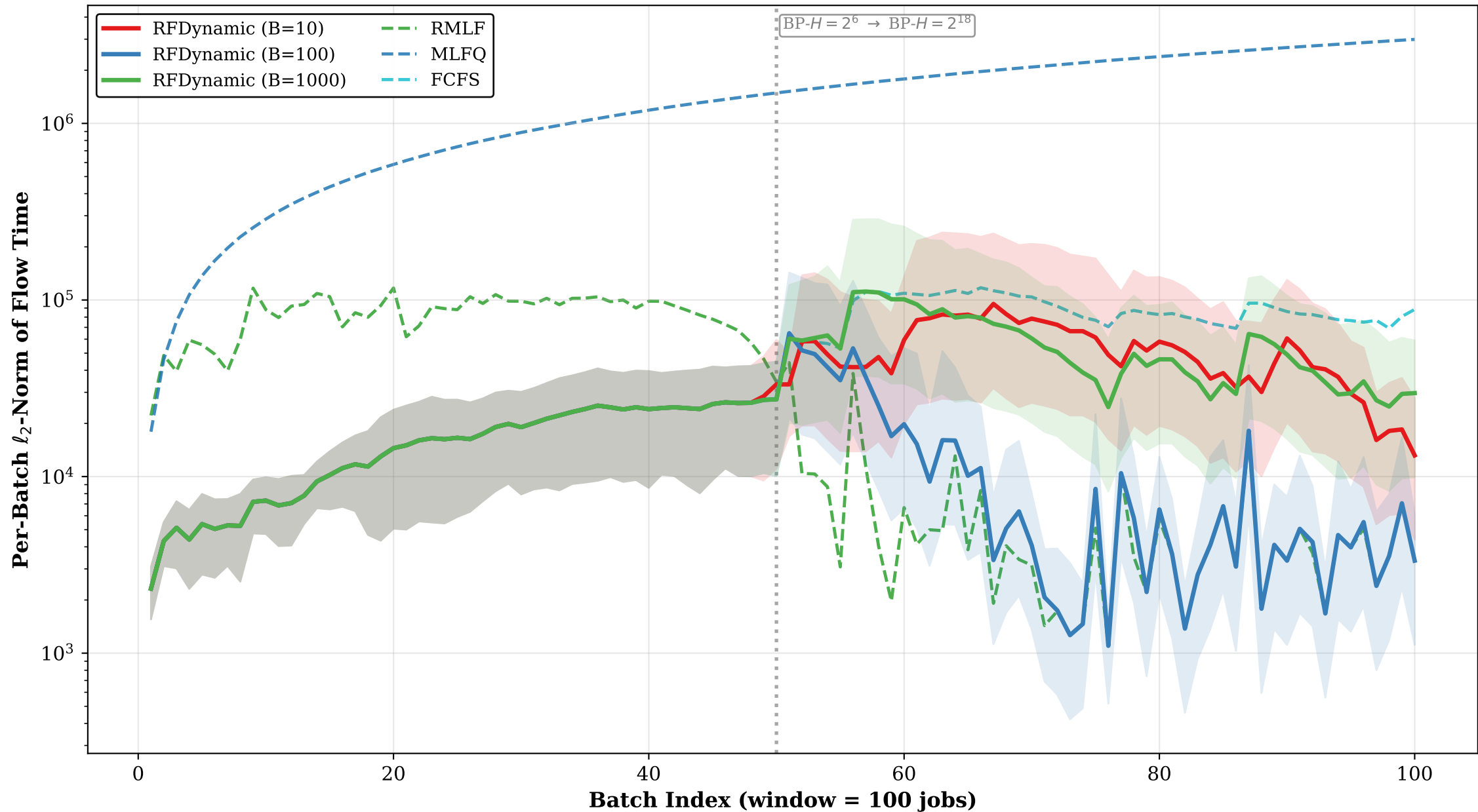
RFDynamic: Distribution Shift ( \text{BP-}H = 2^6 \rightarrow \text{BP-}H = 2^{18} )
