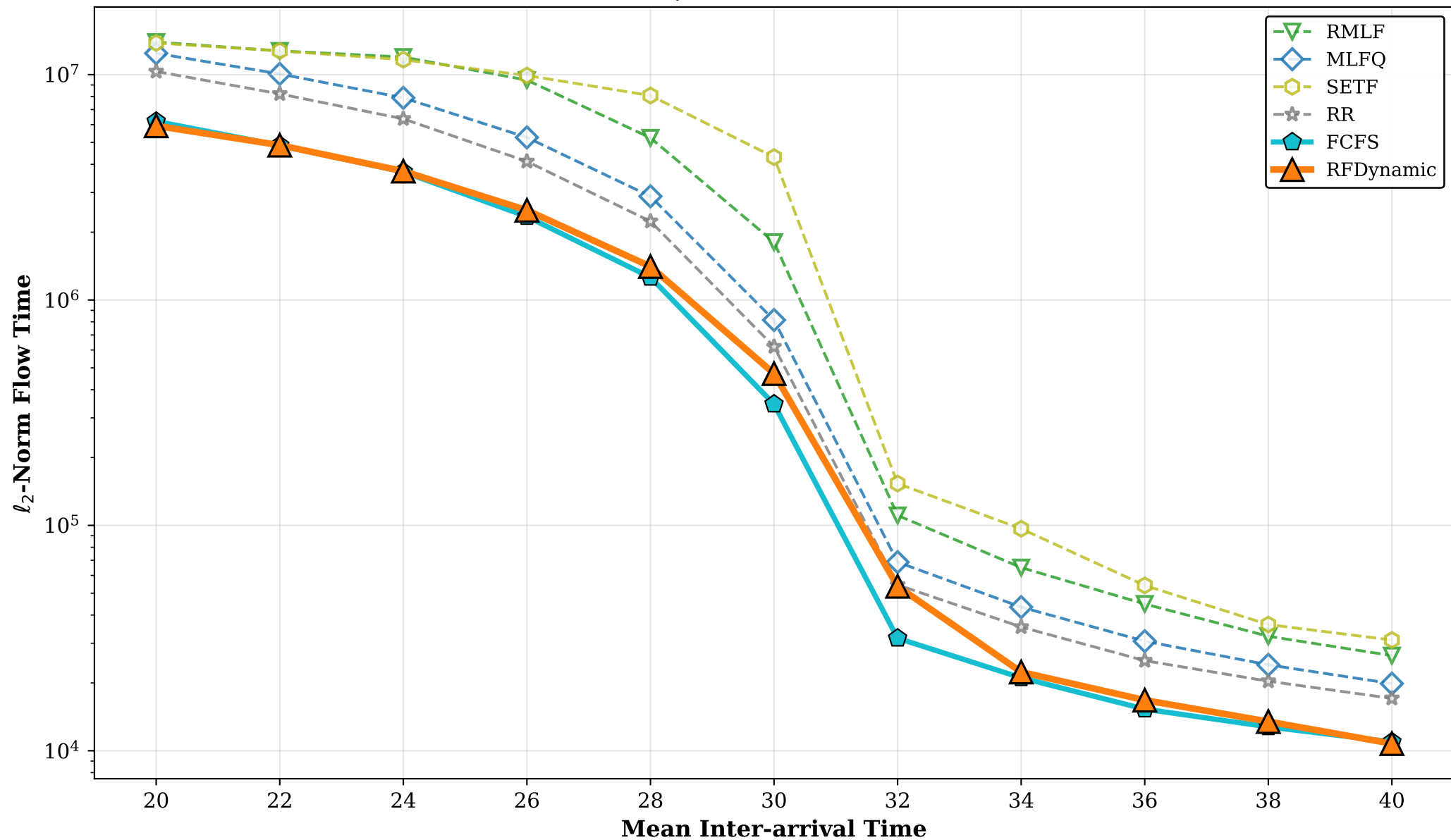
Non-Clairvoyant \ell_2 -Norm Comparison Normal ( \mu = 30, \sigma = 12, CV=0.40 )
