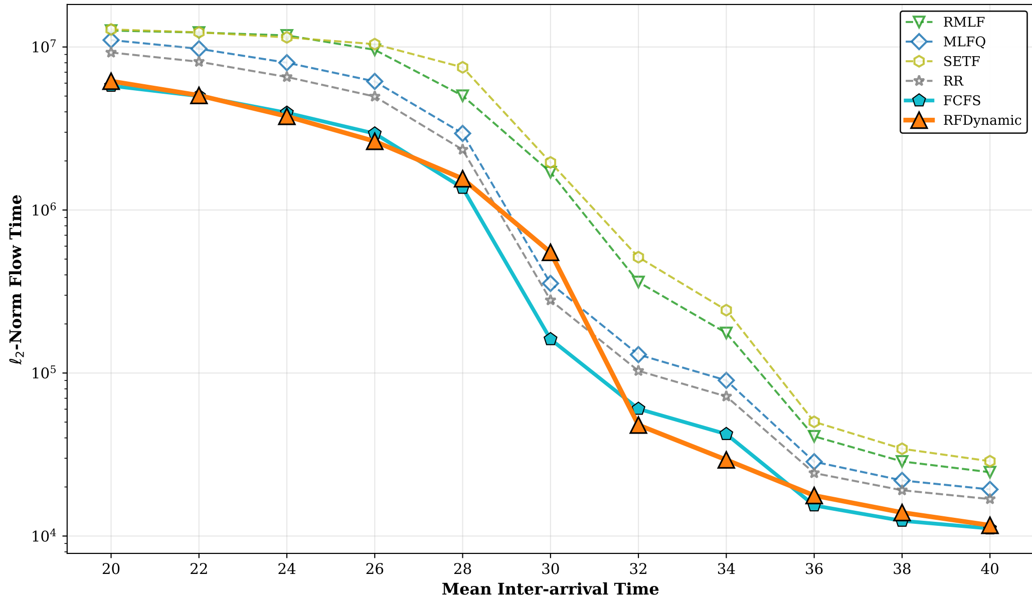
Non-Clairvoyant \ell_2 -Norm Comparison Normal ( \mu = 30, \sigma = 15, CV=0.50 )
