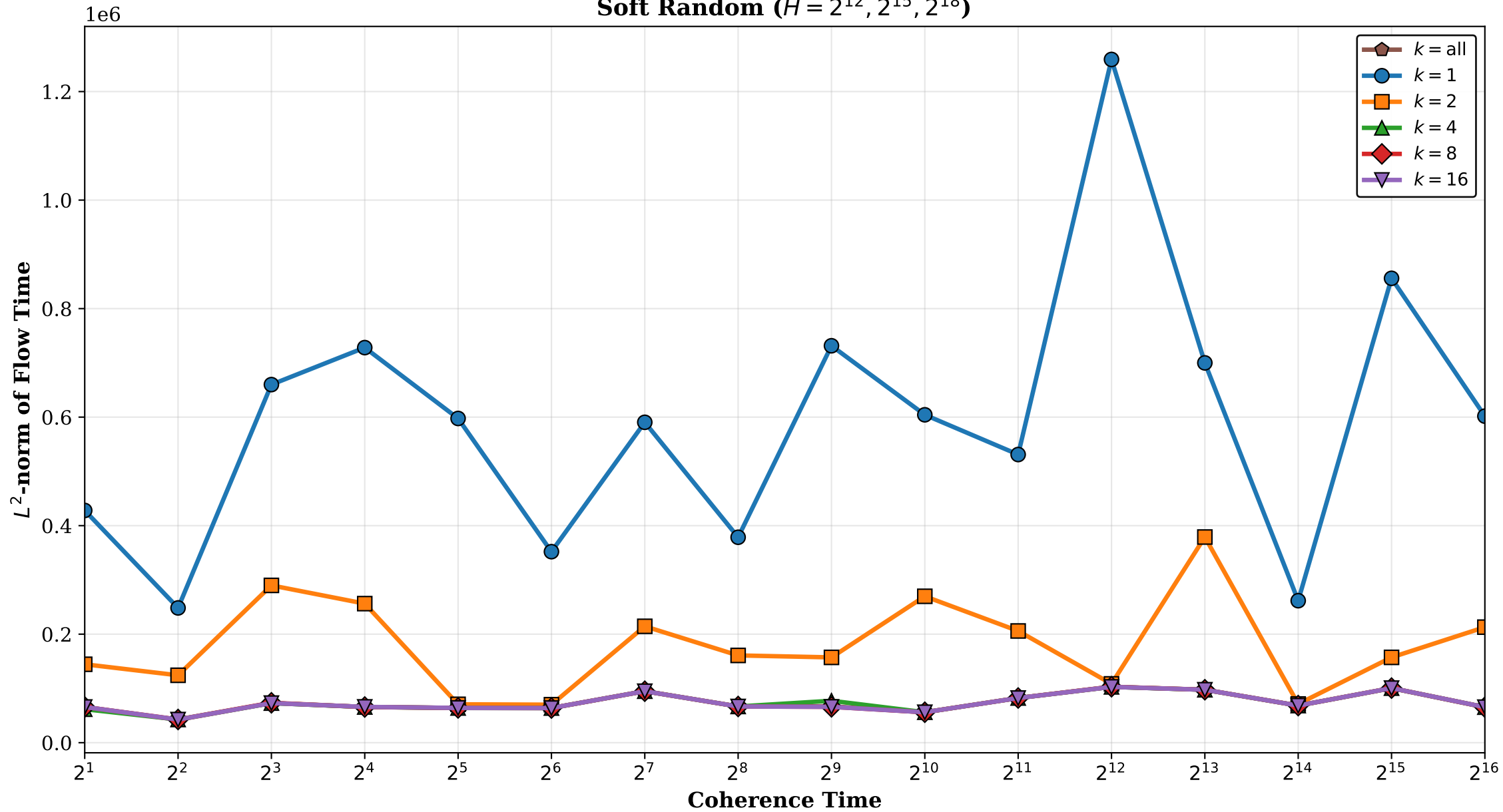
RFDynamic Lookback Comparison Soft Random ( H = 2^{12}, 2^{15}, 2^{18} )
