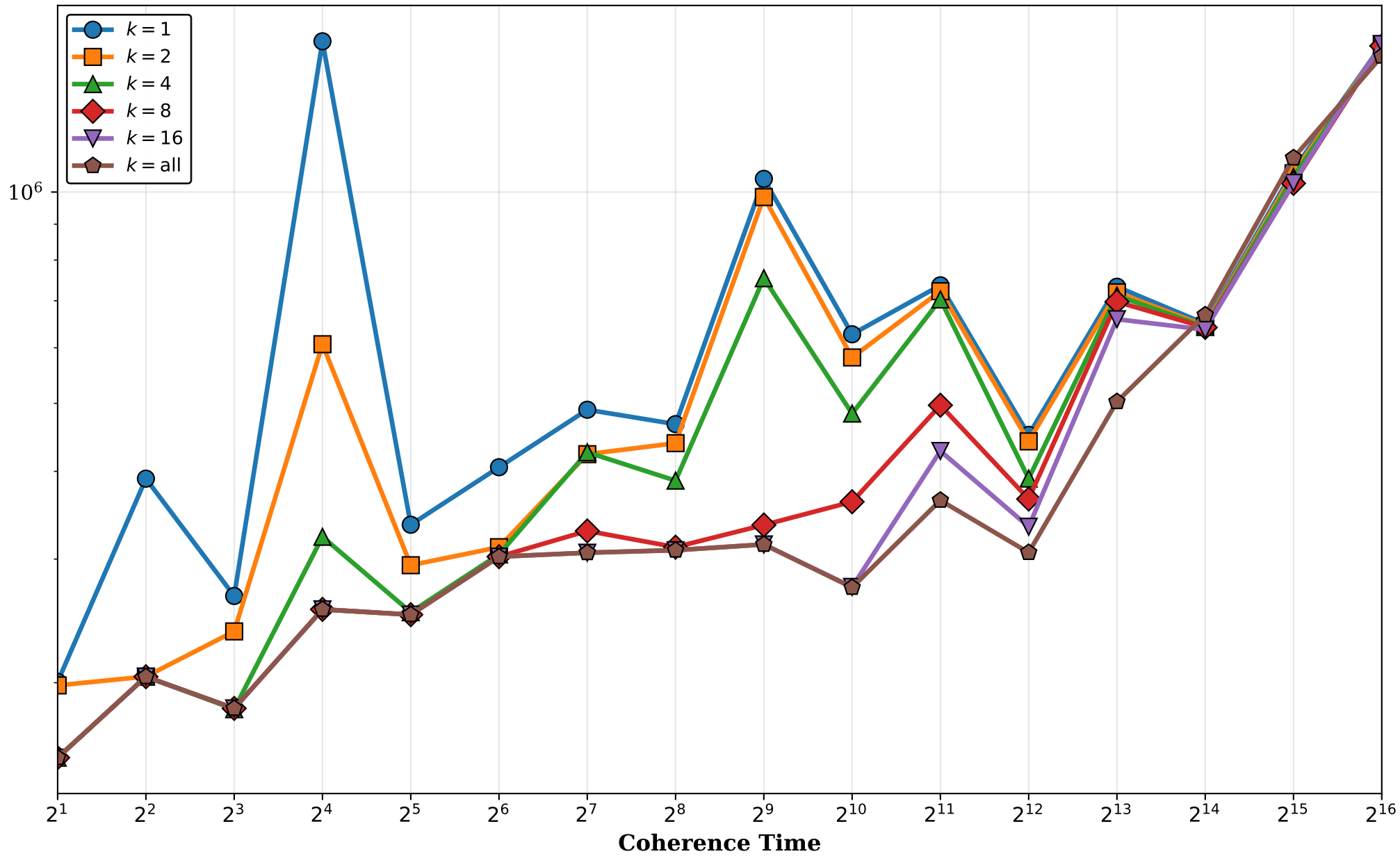
Dynamic Lookback Sensitivity ( B = 100 )
